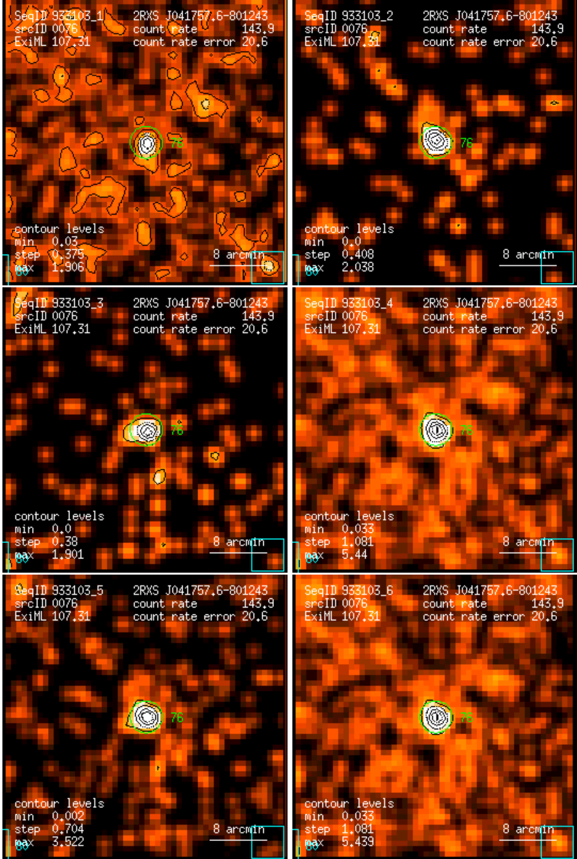
Figure 76: RASS 933103: detection 0076: band rate images, Gaussian filter: (1) PSPC channels 11 – 41, (2) 52 – 90, (3) 91 – 201, (4) 11 – 235, (5) 52 – 201, (6) 11 – 201. Broad band rates in counts/ks. Band rate contour levels in counts/ks/arcmin 2 .
