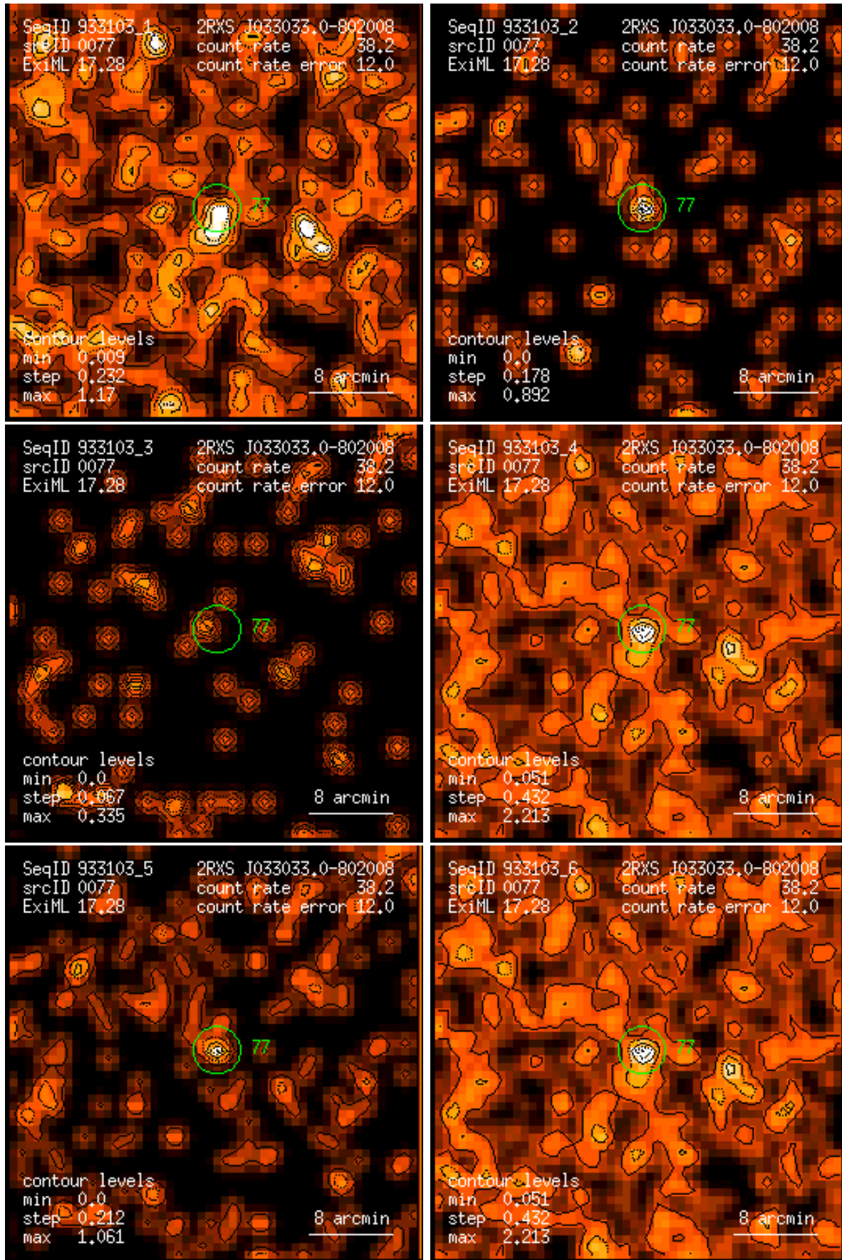
Figure 77: RASS 933103: detection 0077: band rate images, Gaussian filter: (1) PSPC channels 11 – 41, (2) 52 – 90, (3) 91 – 201, (4) 11 – 235, (5) 52 – 201, (6) 11 – 201. Broad band rates in counts/ks. Band rate contour levels in counts/ks/arcmin 2 .
