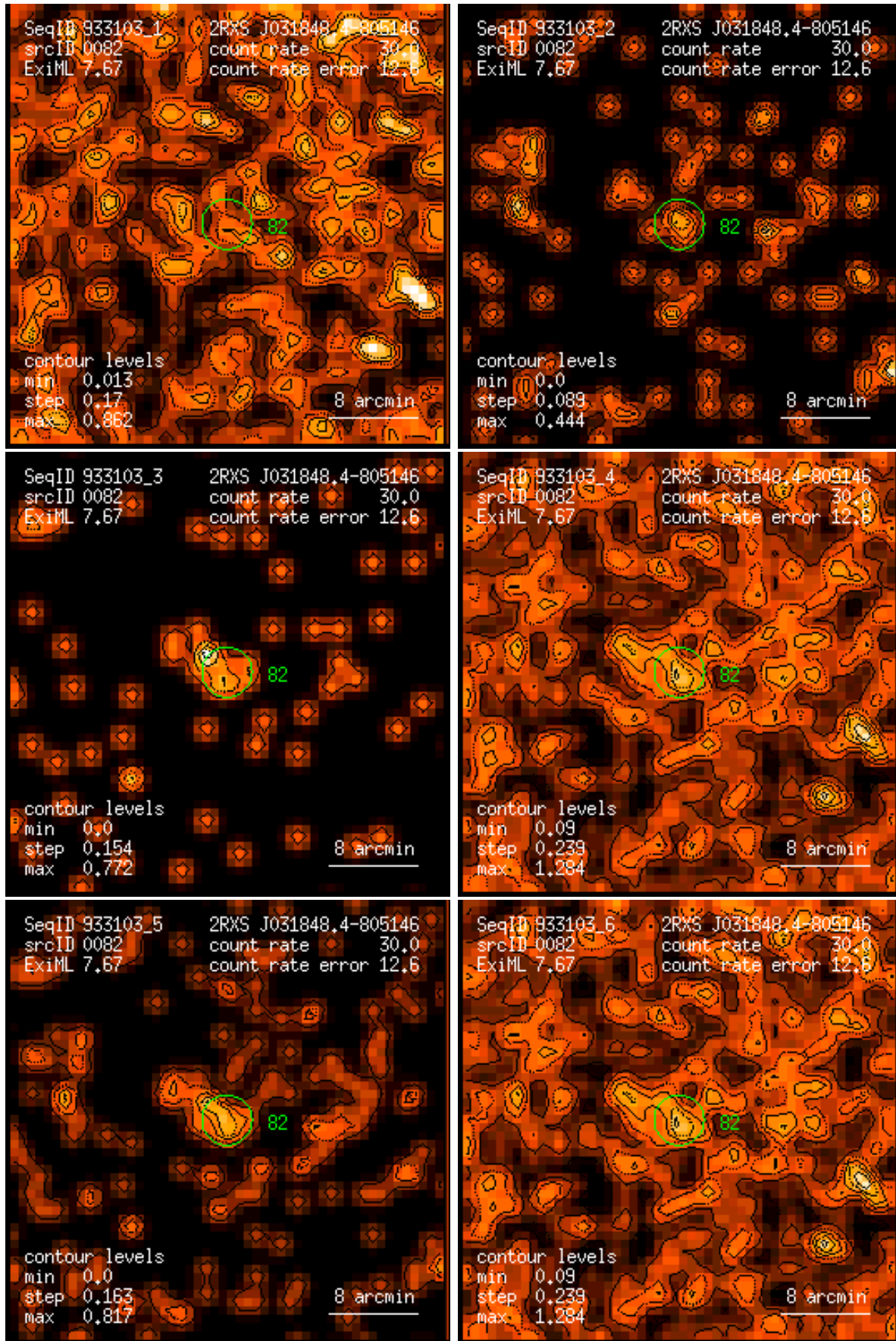
Figure 82: RASS 933103: detection 0082: band rate images, Gaussian filter: (1) PSPC channels 11 – 41, (2) 52 – 90, (3) 91 – 201, (4) 11 – 235, (5) 52 – 201, (6) 11 – 201. Broad band rates in counts/ks. Band rate contour levels in counts/ks/arcmin 2 .
