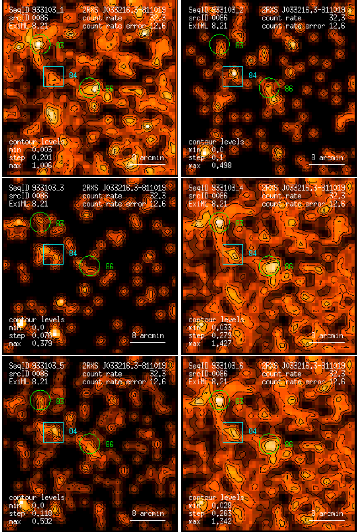
Figure 86: RASS 933103: detection 0086: band rate images, Gaussian filter: (1) PSPC channels 11 – 41, (2) 52 – 90, (3) 91 – 201, (4) 11 – 235, (5) 52 – 201, (6) 11 – 201. Broad band rates in counts/ks. Band rate contour levels in counts/ks/arcmin 2 .
