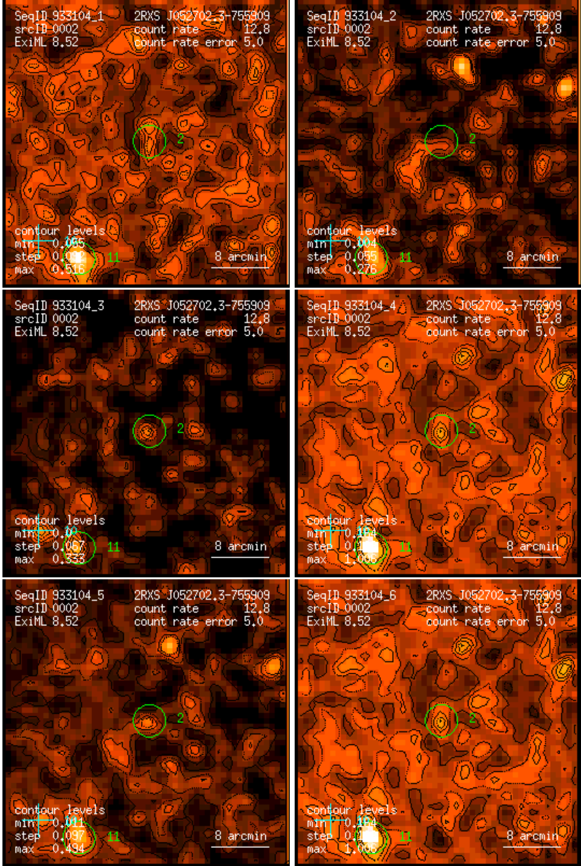
Figure 2: RASS 933104: detection 0002: band rate images, Gaussian filter: (1) PSPC channels 11 – 41, (2) 52 – 90, (3) 91 – 201, (4) 11 – 235, (5) 52 – 201, (6) 11 – 201. Broad band rates in counts/ks. Band rate contour levels in counts/ks/arcmin 2 .
