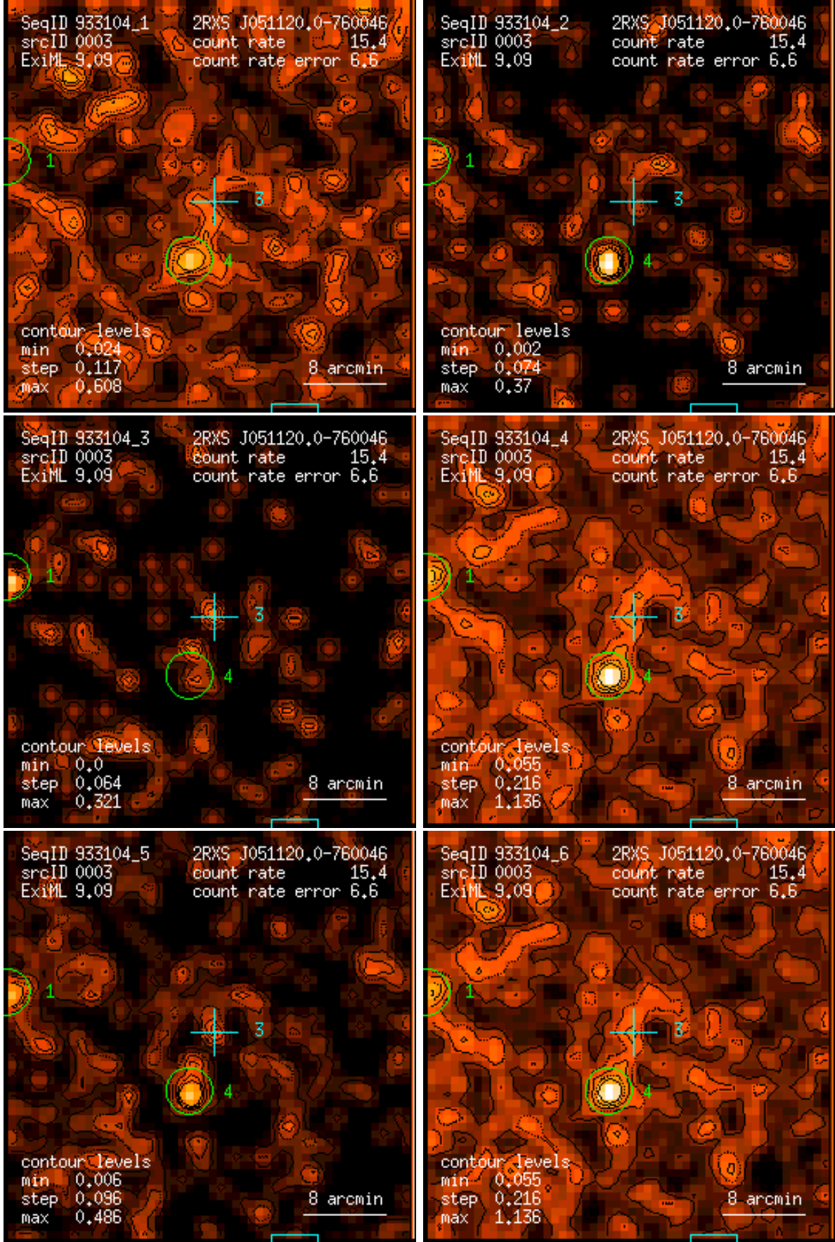
Figure 3: RASS 933104: detection 0003: band rate images, Gaussian filter: (1) PSPC channels 11 – 41, (2) 52 – 90, (3) 91 – 201, (4) 11 – 235, (5) 52 – 201, (6) 11 – 201. Broad band rates in counts/ks. Band rate contour levels in counts/ks/arcmin 2 .
