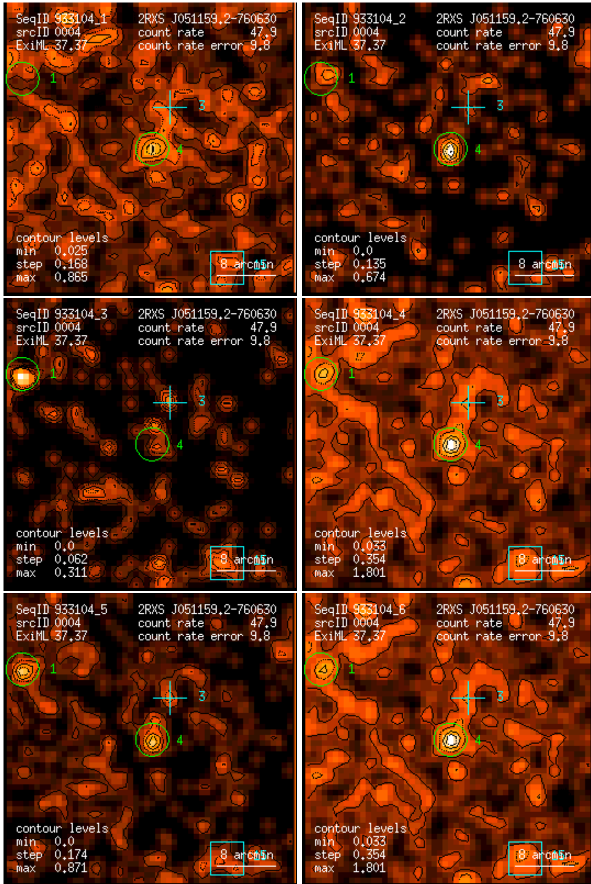
Figure 4: RASS 933104: detection 0004: band rate images, Gaussian filter: (1) PSPC channels 11 – 41, (2) 52 – 90, (3) 91 – 201, (4) 11 – 235, (5) 52 – 201, (6) 11 – 201. Broad band rates in counts/ks. Band rate contour levels in counts/ks/arcmin 2 .
