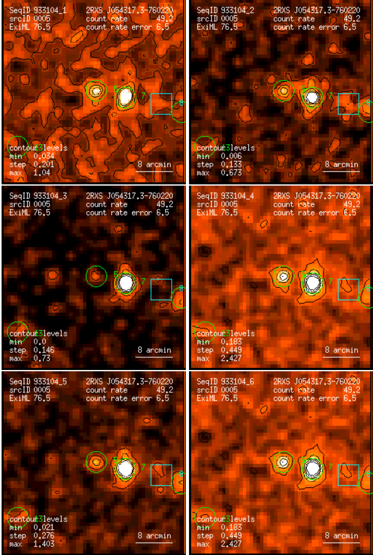
Figure 5: RASS 933104: detection 0005: band rate images, Gaussian filter: (1) PSPC channels 11 – 41, (2) 52 – 90, (3) 91 – 201, (4) 11 – 235, (5) 52 – 201, (6) 11 – 201. Broad band rates in counts/ks. Band rate contour levels in counts/ks/arcmin 2 .
