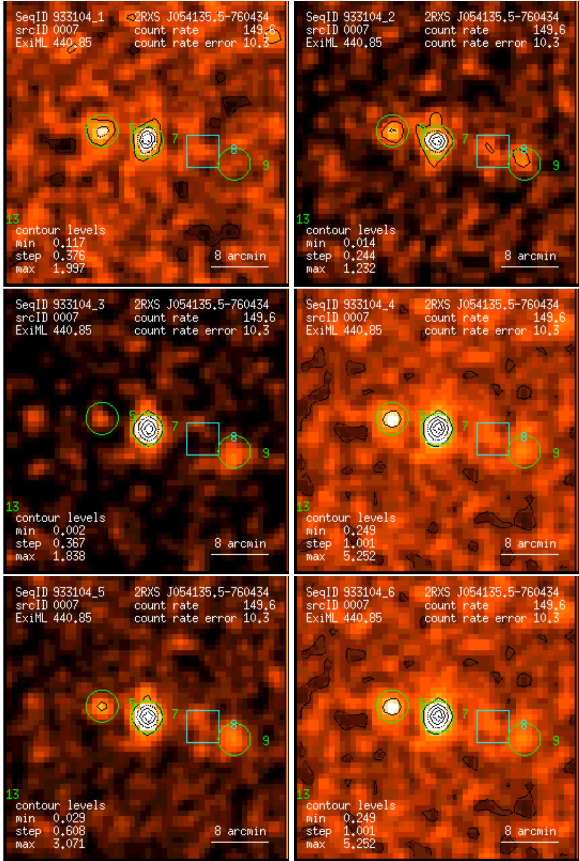
Figure 7: RASS 933104: detection 0007: band rate images, Gaussian filter: (1) PSPC channels 11 – 41, (2) 52 – 90, (3) 91 – 201, (4) 11 – 235, (5) 52 – 201, (6) 11 – 201. Broad band rates in counts/ks. Band rate contour levels in counts/ks/arcmin 2 .
