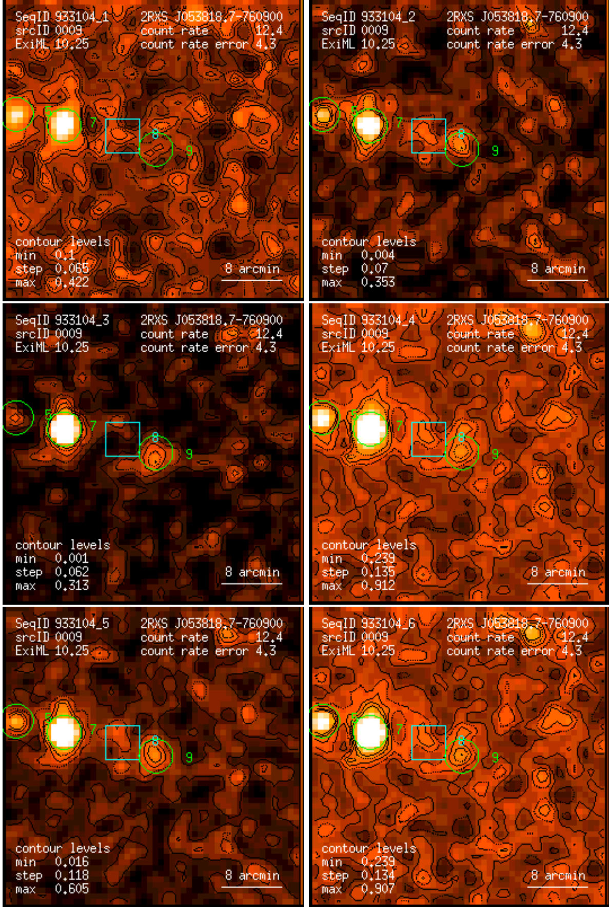
Figure 9: RASS 933104: detection 0009: band rate images, Gaussian filter: (1) PSPC channels 11 – 41, (2) 52 – 90, (3) 91 – 201, (4) 11 – 235, (5) 52 – 201, (6) 11 – 201. Broad band rates in counts/ks. Band rate contour levels in counts/ks/arcmin 2 .
