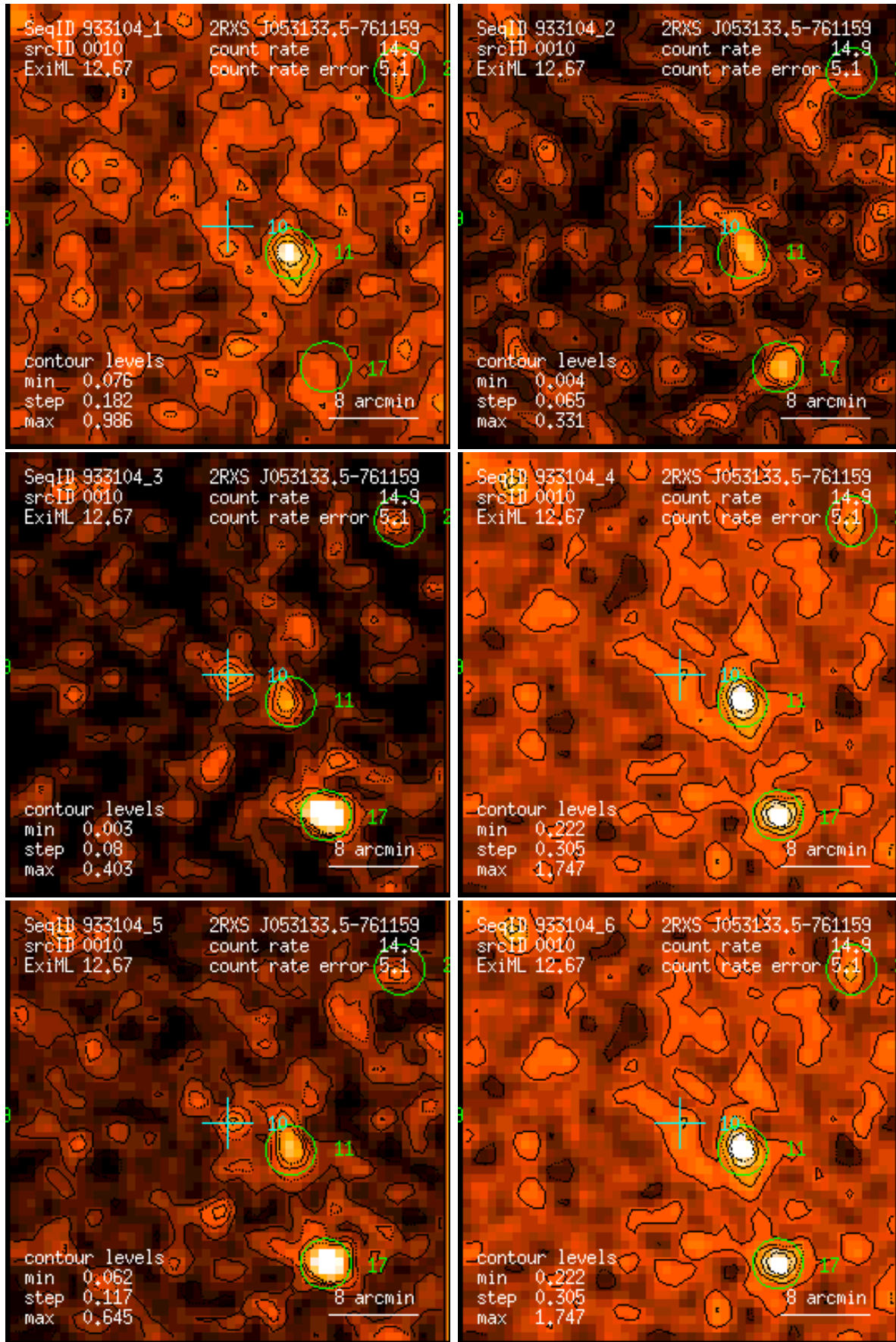
Figure 10: RASS 933104: detection 0010: band rate images, Gaussian filter: (1) PSPC channels 11 – 41, (2) 52 – 90, (3) 91 – 201, (4) 11 – 235, (5) 52 – 201, (6) 11 – 201. Broad band rates in counts/ks. Band rate contour levels in counts/ks/arcmin 2 .
