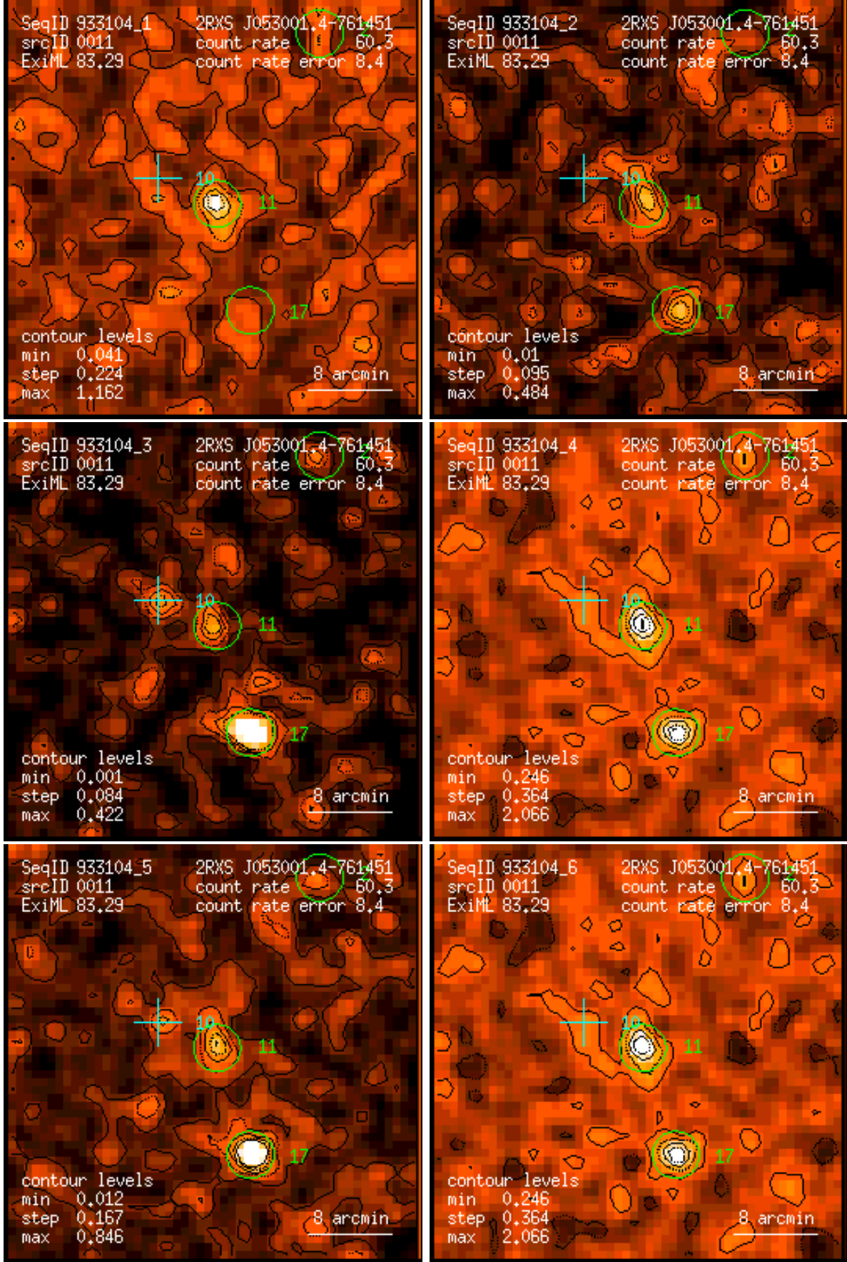
Figure 11: RASS 933104: detection 0011: band rate images, Gaussian filter: (1) PSPC channels 11 – 41, (2) 52 – 90, (3) 91 – 201, (4) 11 – 235, (5) 52 – 201, (6) 11 – 201. Broad band rates in counts/ks. Band rate contour levels in counts/ks/arcmin 2 .
