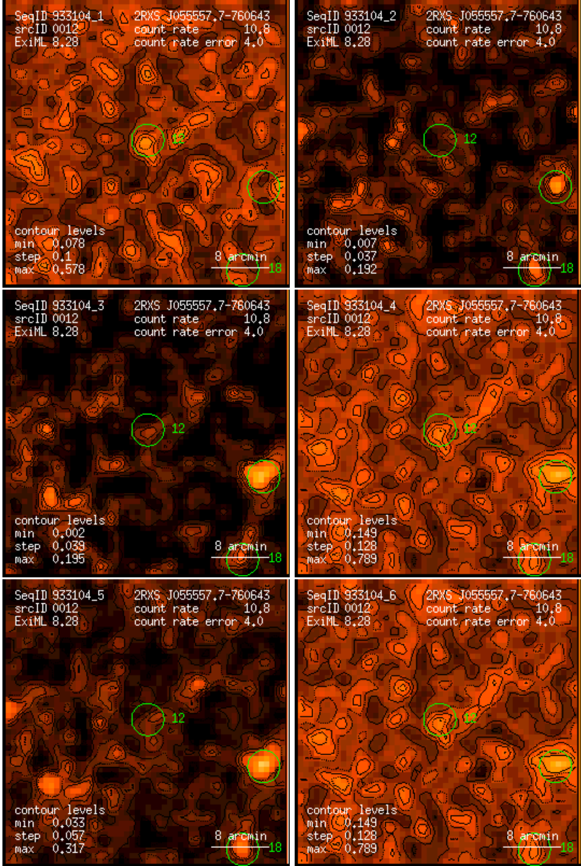
Figure 12: RASS 933104: detection 0012: band rate images, Gaussian filter: (1) PSPC channels 11 – 41, (2) 52 – 90, (3) 91 – 201, (4) 11 – 235, (5) 52 – 201, (6) 11 – 201. Broad band rates in counts/ks. Band rate contour levels in counts/ks/arcmin 2 .
