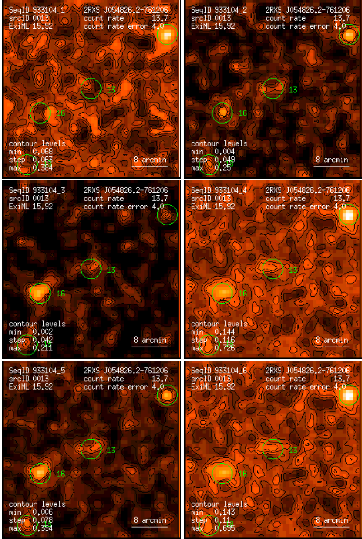
Figure 13: RASS 933104: detection 0013: band rate images, Gaussian filter: (1) PSPC channels 11 – 41, (2) 52 – 90, (3) 91 – 201, (4) 11 – 235, (5) 52 – 201, (6) 11 – 201. Broad band rates in counts/ks. Band rate contour levels in counts/ks/arcmin 2 .
