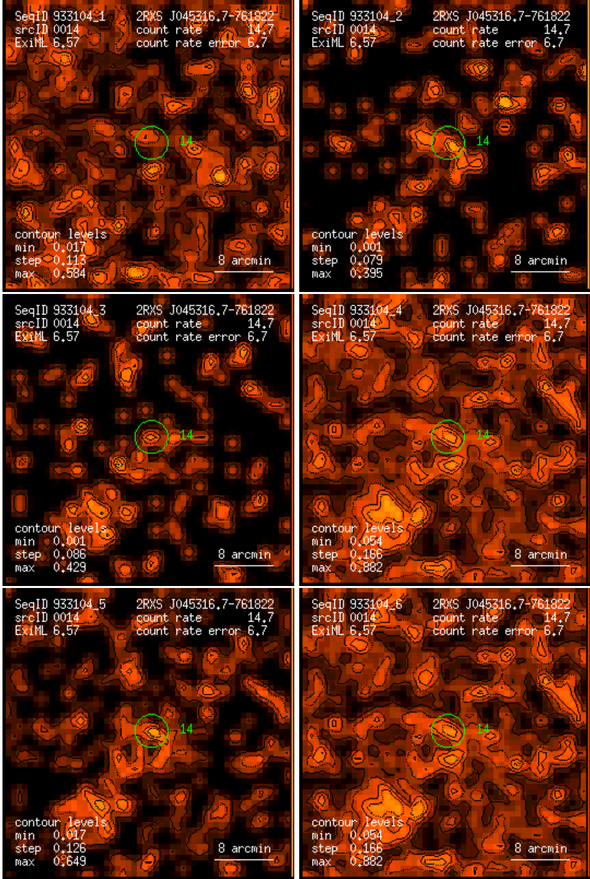
Figure 14: RASS 933104: detection 0014: band rate images, Gaussian filter: (1) PSPC channels 11 – 41, (2) 52 – 90, (3) 91 – 201, (4) 11 – 235, (5) 52 – 201, (6) 11 – 201. Broad band rates in counts/ks. Band rate contour levels in counts/ks/arcmin 2 .
