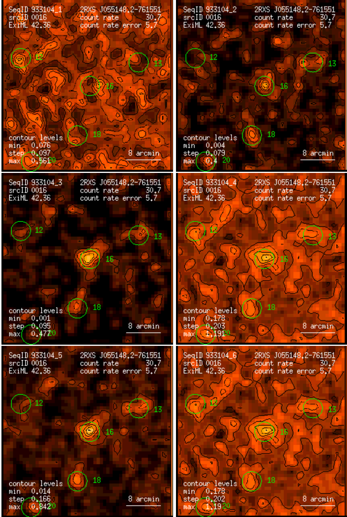
Figure 16: RASS 933104: detection 0016: band rate images, Gaussian filter: (1) PSPC channels 11 – 41, (2) 52 – 90, (3) 91 – 201, (4) 11 – 235, (5) 52 – 201, (6) 11 – 201. Broad band rates in counts/ks. Band rate contour levels in counts/ks/arcmin 2 .
