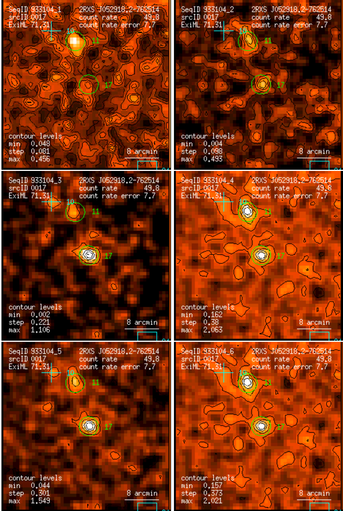
Figure 17: RASS 933104: detection 0017: band rate images, Gaussian filter: (1) PSPC channels 11 – 41, (2) 52 – 90, (3) 91 – 201, (4) 11 – 235, (5) 52 – 201, (6) 11 – 201. Broad band rates in counts/ks. Band rate contour levels in counts/ks/arcmin 2 .
