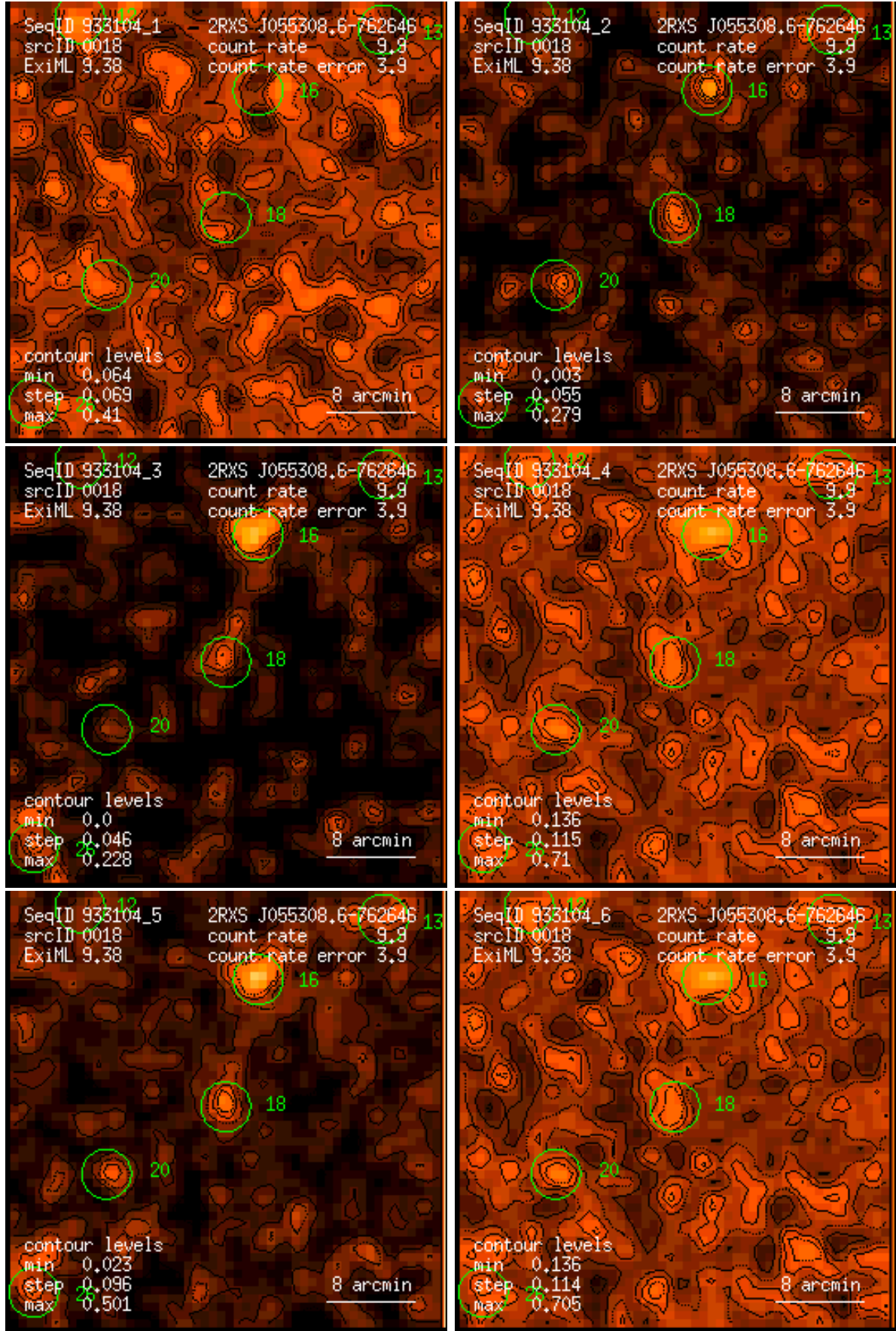
Figure 18: RASS 933104: detection 0018: band rate images, Gaussian filter: (1) PSPC channels 11 – 41, (2) 52 – 90, (3) 91 – 201, (4) 11 – 235, (5) 52 – 201, (6) 11 – 201. Broad band rates in counts/ks. Band rate contour levels in counts/ks/arcmin 2 .
