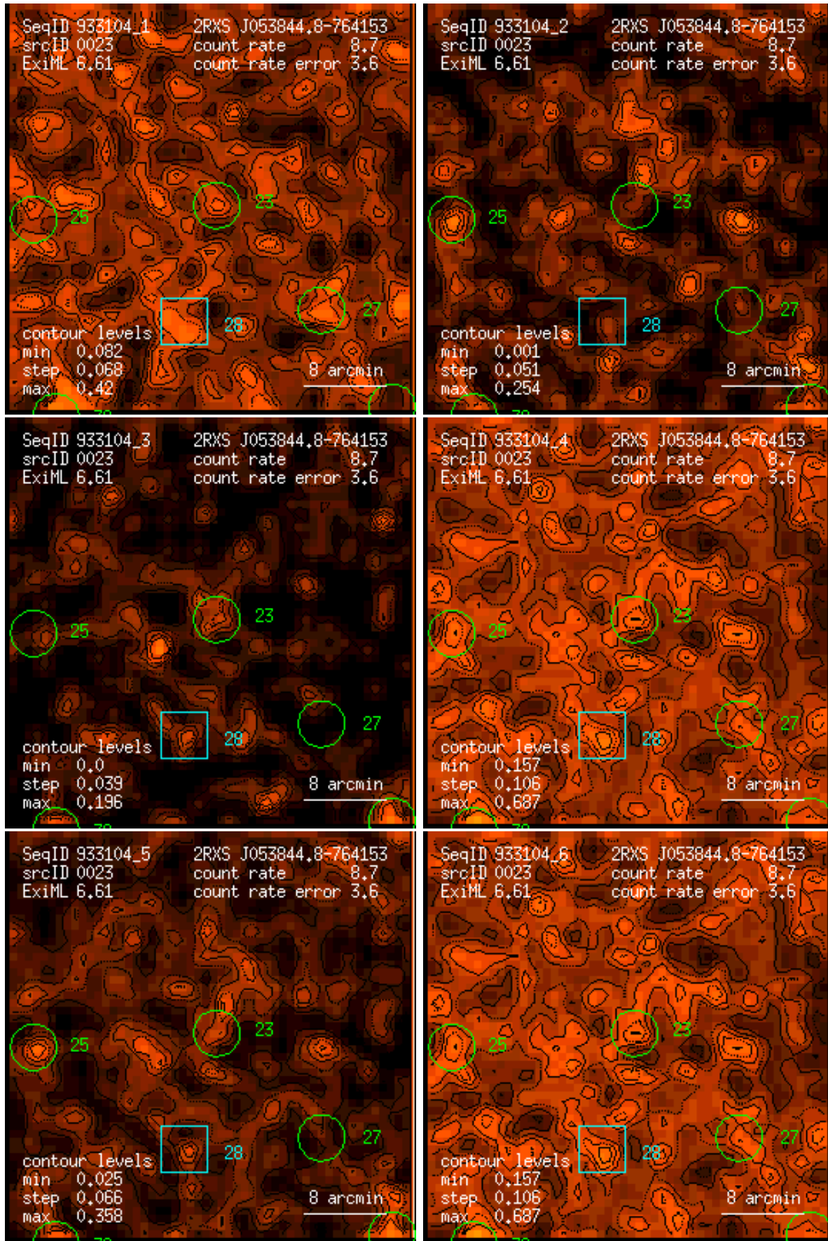
Figure 23: RASS 933104: detection 0023: band rate images, Gaussian filter: (1) PSPC channels 11 – 41, (2) 52 – 90, (3) 91 – 201, (4) 11 – 235, (5) 52 – 201, (6) 11 – 201. Broad band rates in counts/ks. Band rate contour levels in counts/ks/arcmin 2 .
