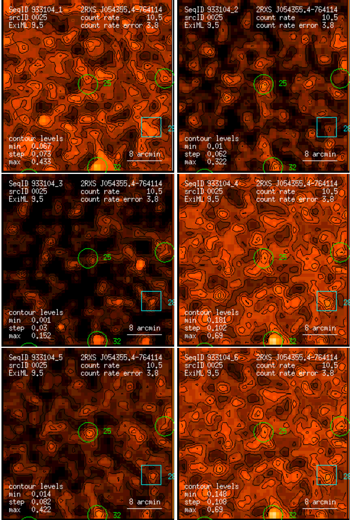
Figure 25: RASS 933104: detection 0025: band rate images, Gaussian filter: (1) PSPC channels 11 – 41, (2) 52 – 90, (3) 91 – 201, (4) 11 – 235, (5) 52 – 201, (6) 11 – 201. Broad band rates in counts/ks. Band rate contour levels in counts/ks/arcmin 2 .
