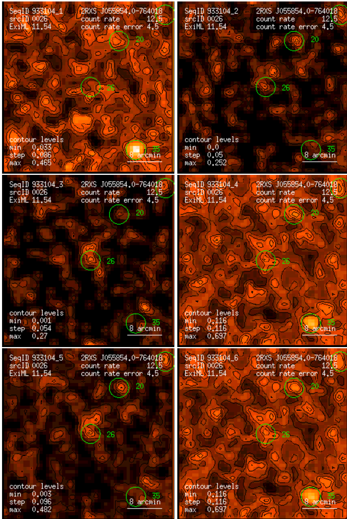
Figure 26: RASS 933104: detection 0026: band rate images, Gaussian filter: (1) PSPC channels 11 – 41, (2) 52 – 90, (3) 91 – 201, (4) 11 – 235, (5) 52 – 201, (6) 11 – 201. Broad band rates in counts/ks. Band rate contour levels in counts/ks/arcmin 2 .
