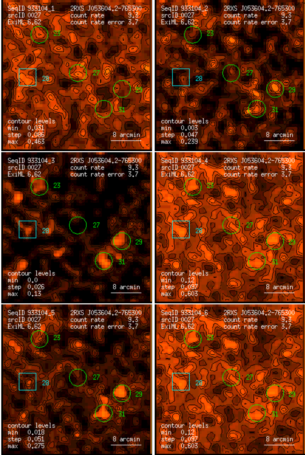
Figure 27: RASS 933104: detection 0027: band rate images, Gaussian filter: (1) PSPC channels 11 – 41, (2) 52 – 90, (3) 91 – 201, (4) 11 – 235, (5) 52 – 201, (6) 11 – 201. Broad band rates in counts/ks. Band rate contour levels in counts/ks/arcmin 2 .
