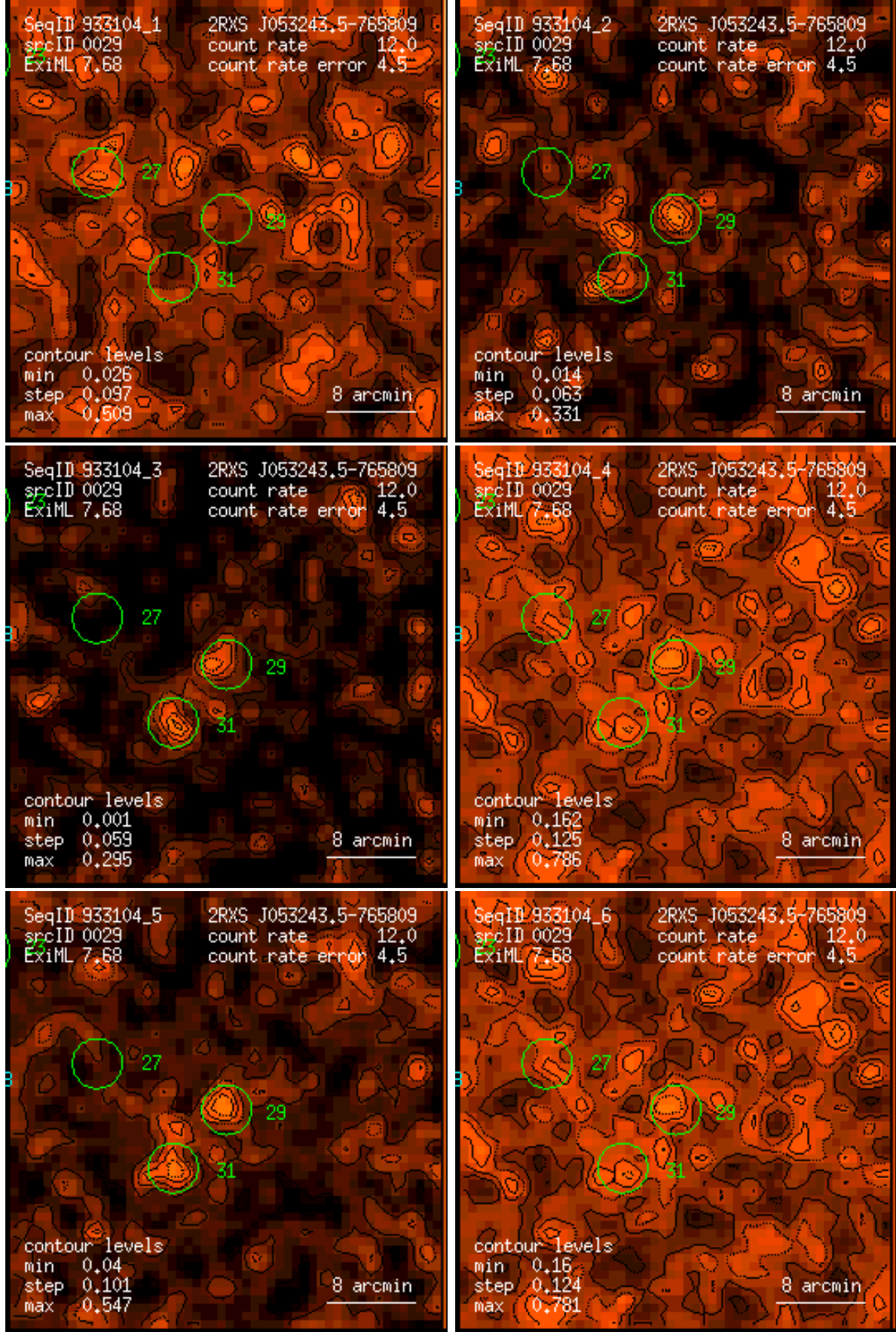
Figure 29: RASS 933104: detection 0029: band rate images, Gaussian filter: (1) PSPC channels 11 – 41, (2) 52 – 90, (3) 91 – 201, (4) 11 – 235, (5) 52 – 201, (6) 11 – 201. Broad band rates in counts/ks. Band rate contour levels in counts/ks/arcmin 2 .
