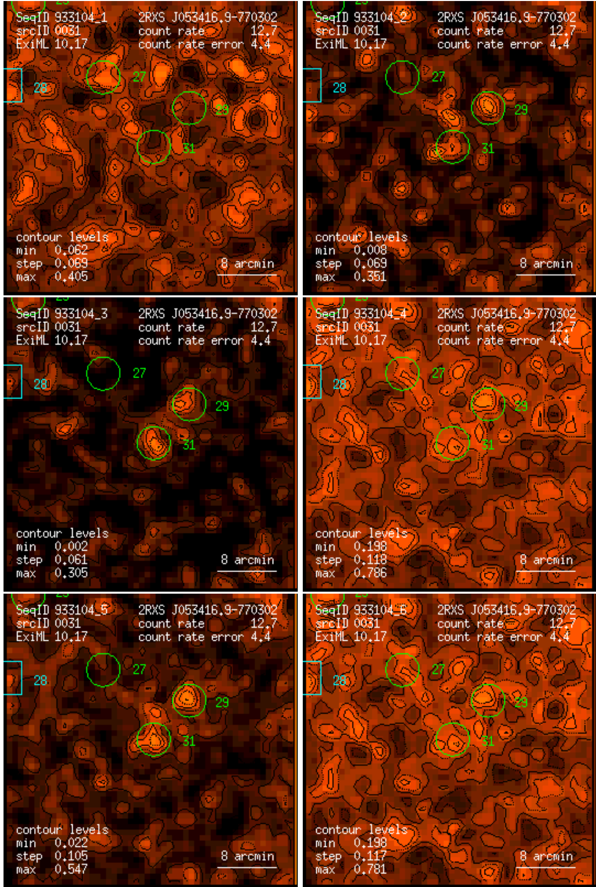
Figure 31: RASS 933104: detection 0031: band rate images, Gaussian filter: (1) PSPC channels 11 – 41, (2) 52 – 90, (3) 91 – 201, (4) 11 – 235, (5) 52 – 201, (6) 11 – 201. Broad band rates in counts/ks. Band rate contour levels in counts/ks/arcmin 2 .
