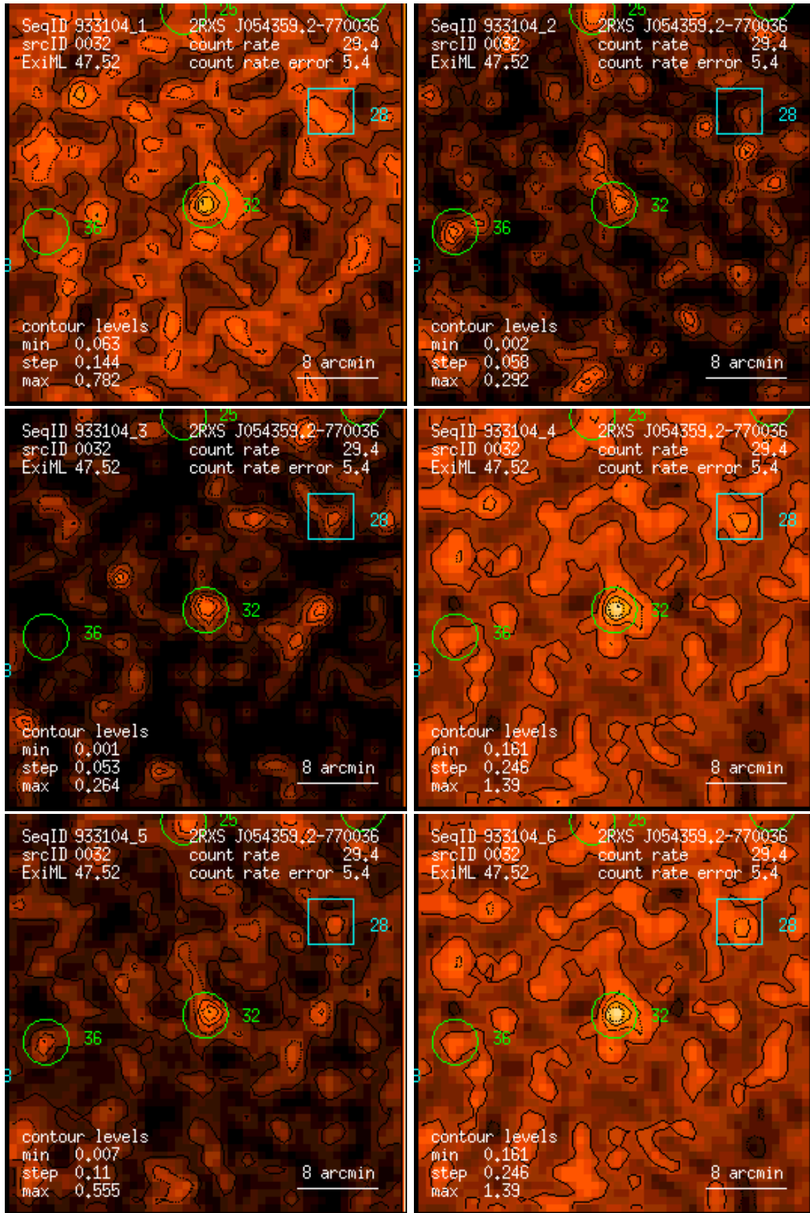
Figure 32: RASS 933104: detection 0032: band rate images, Gaussian filter: (1) PSPC channels 11 – 41, (2) 52 – 90, (3) 91 – 201, (4) 11 – 235, (5) 52 – 201, (6) 11 – 201. Broad band rates in counts/ks. Band rate contour levels in counts/ks/arcmin 2 .
