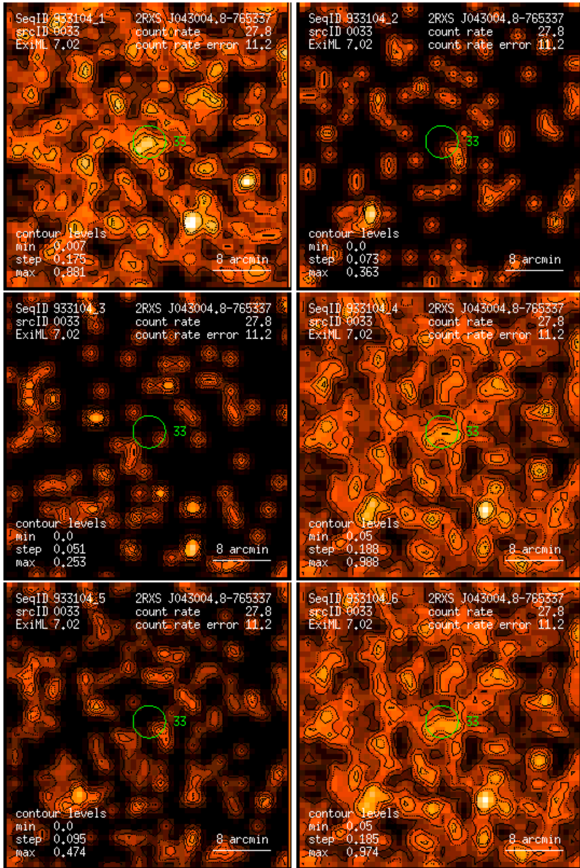
Figure 33: RASS 933104: detection 0033: band rate images, Gaussian filter: (1) PSPC channels 11 – 41, (2) 52 – 90, (3) 91 – 201, (4) 11 – 235, (5) 52 – 201, (6) 11 – 201. Broad band rates in counts/ks. Band rate contour levels in counts/ks/arcmin 2 .
