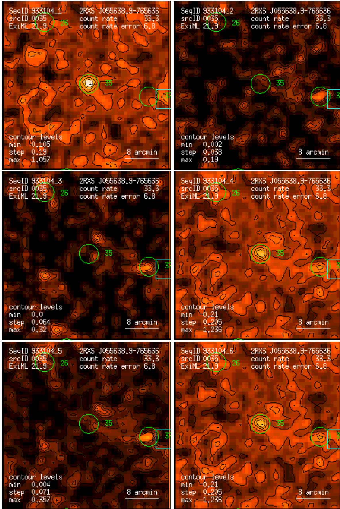
Figure 35: RASS 933104: detection 0035: band rate images, Gaussian filter: (1) PSPC channels 11 – 41, (2) 52 – 90, (3) 91 – 201, (4) 11 – 235, (5) 52 – 201, (6) 11 – 201. Broad band rates in counts/ks. Band rate contour levels in counts/ks/arcmin 2 .
