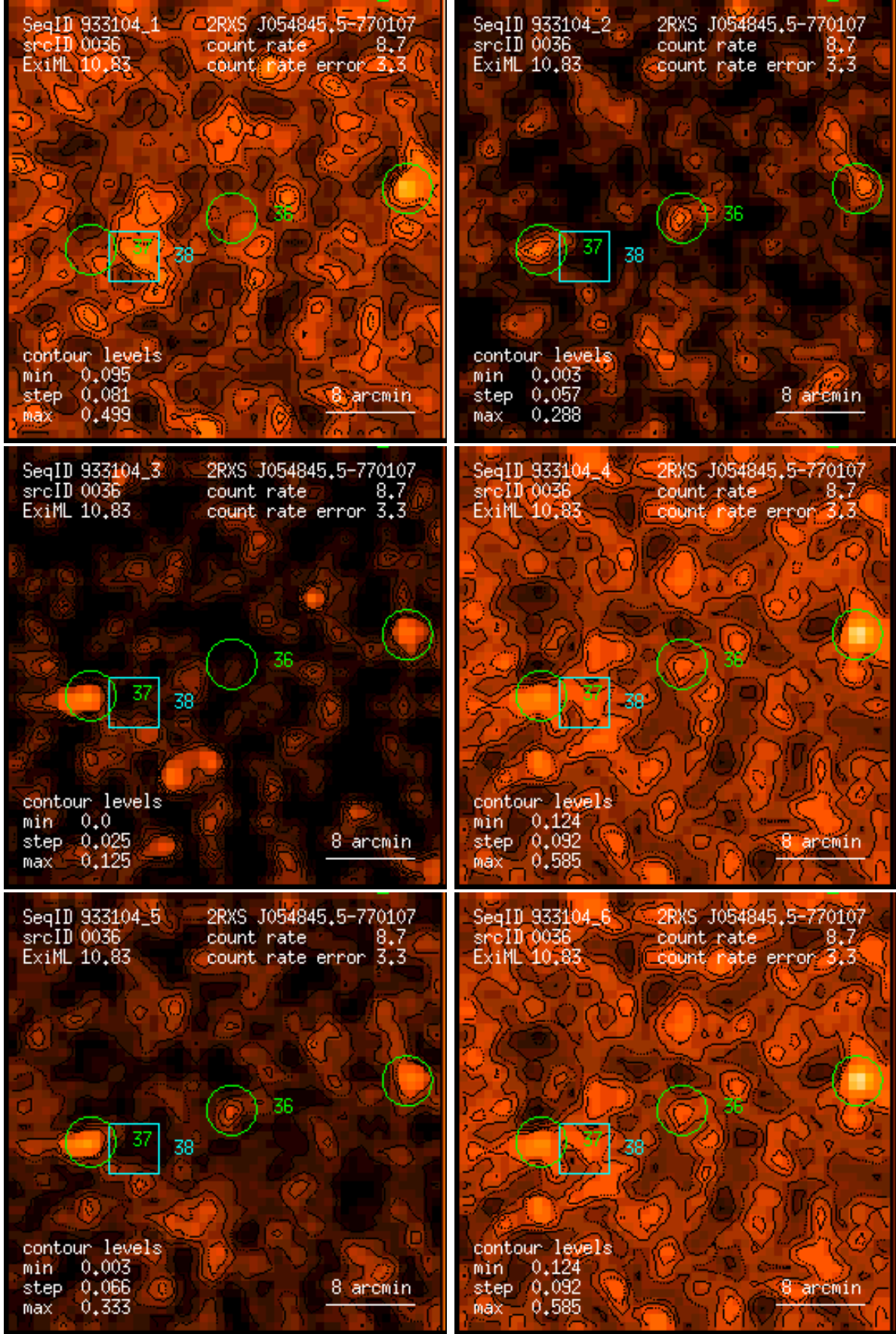
Figure 36: RASS 933104: detection 0036: band rate images, Gaussian filter: (1) PSPC channels 11 – 41, (2) 52 – 90, (3) 91 – 201, (4) 11 – 235, (5) 52 – 201, (6) 11 – 201. Broad band rates in counts/ks. Band rate contour levels in counts/ks/arcmin 2 .
