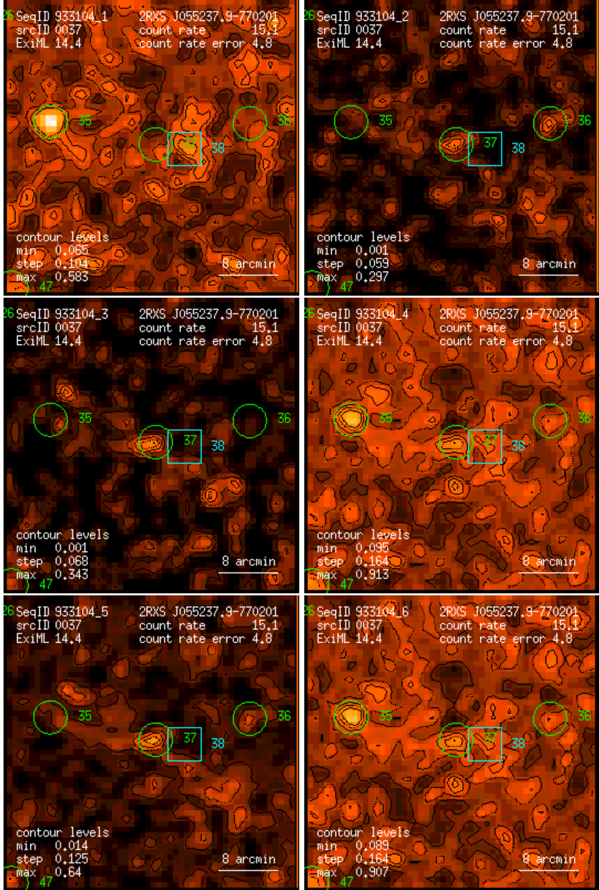
Figure 37: RASS 933104: detection 0037: band rate images, Gaussian filter: (1) PSPC channels 11 – 41, (2) 52 – 90, (3) 91 – 201, (4) 11 – 235, (5) 52 – 201, (6) 11 – 201. Broad band rates in counts/ks. Band rate contour levels in counts/ks/arcmin 2 .
