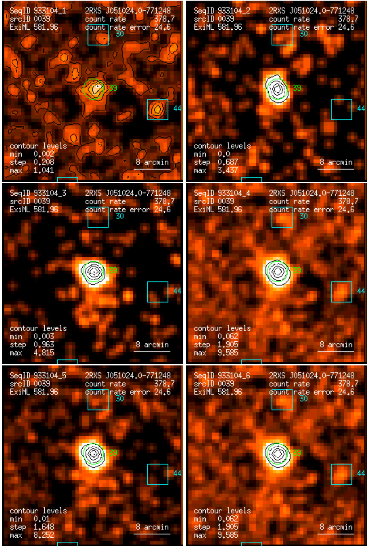
Figure 39: RASS 933104: detection 0039: band rate images, Gaussian filter: (1) PSPC channels 11 – 41, (2) 52 – 90, (3) 91 – 201, (4) 11 – 235, (5) 52 – 201, (6) 11 – 201. Broad band rates in counts/ks. Band rate contour levels in counts/ks/arcmin 2 .
