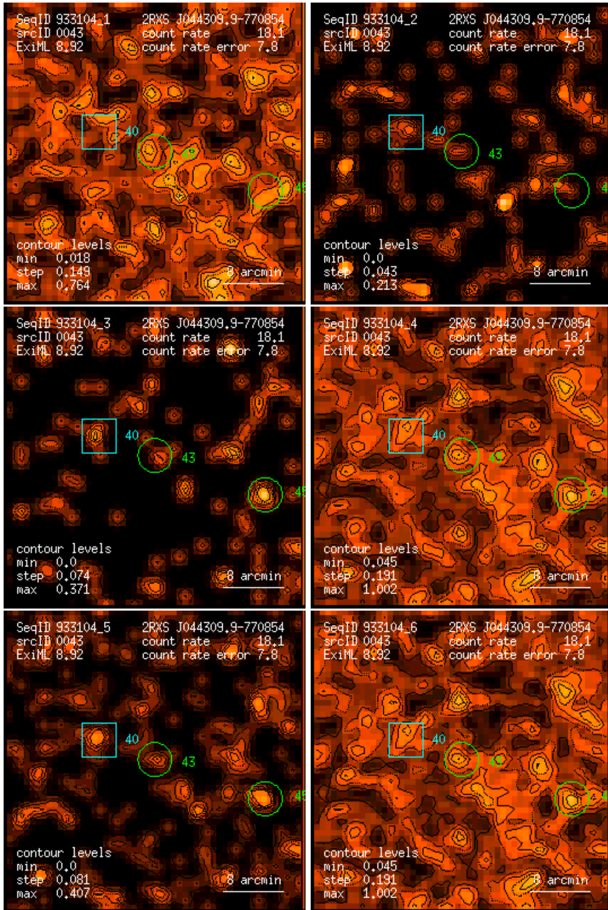
Figure 43: RASS 933104: detection 0043: band rate images, Gaussian filter: (1) PSPC channels 11 – 41, (2) 52 – 90, (3) 91 – 201, (4) 11 – 235, (5) 52 – 201, (6) 11 – 201. Broad band rates in counts/ks. Band rate contour levels in counts/ks/arcmin 2 .
