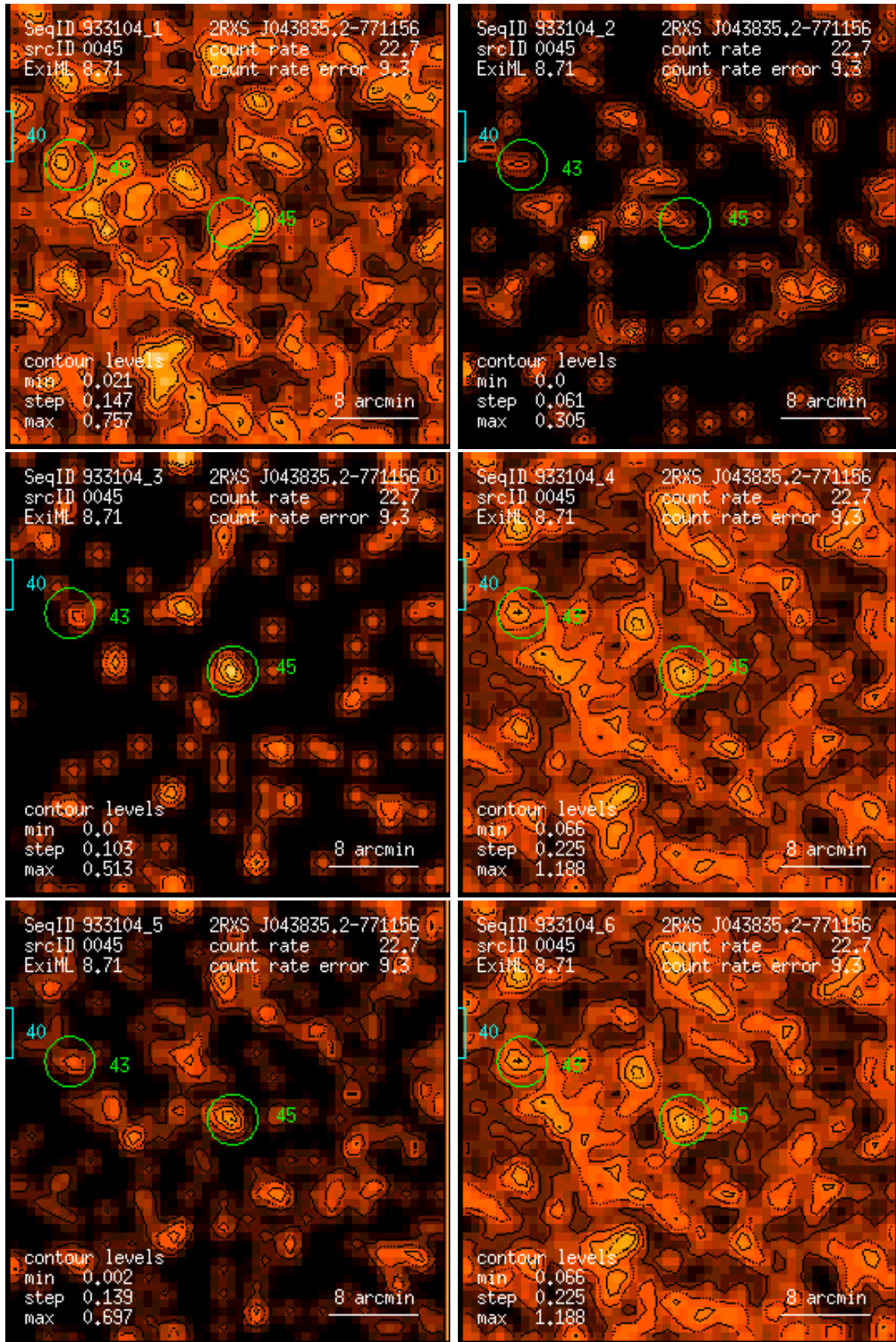
Figure 45: RASS 933104: detection 0045: band rate images, Gaussian filter: (1) PSPC channels 11 – 41, (2) 52 – 90, (3) 91 – 201, (4) 11 – 235, (5) 52 – 201, (6) 11 – 201. Broad band rates in counts/ks. Band rate contour levels in counts/ks/arcmin 2 .
