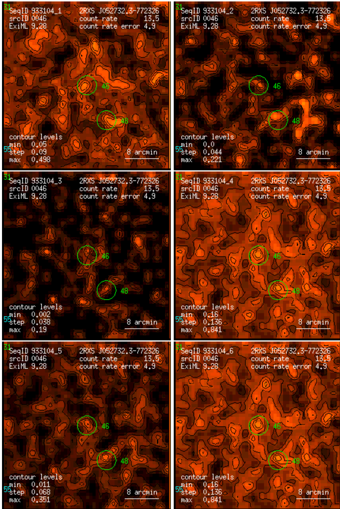
Figure 46: RASS 933104: detection 0046: band rate images, Gaussian filter: (1) PSPP channels 11 – 41, (2) 52 – 90, (3) 91 – 201, (4) 11 – 235, (5) 52 – 201, (6) 11 – 201. Broad band rates in counts/ks. Band rate contour levels in counts/ks/arcmin 2 .
