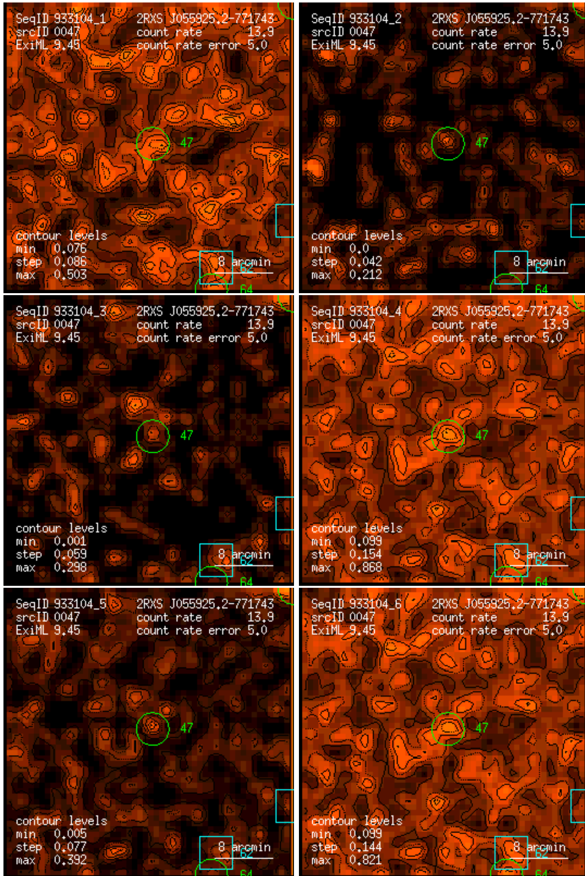
Figure 47: RASS 933104: detection 0047: band rate images, Gaussian filter: (1) PSPC channels 11 – 41, (2) 52 – 90, (3) 91 – 201, (4) 11 – 235, (5) 52 – 201, (6) 11 – 201. Broad band rates in counts/ks. Band rate contour levels in counts/ks/arcmin 2 .
