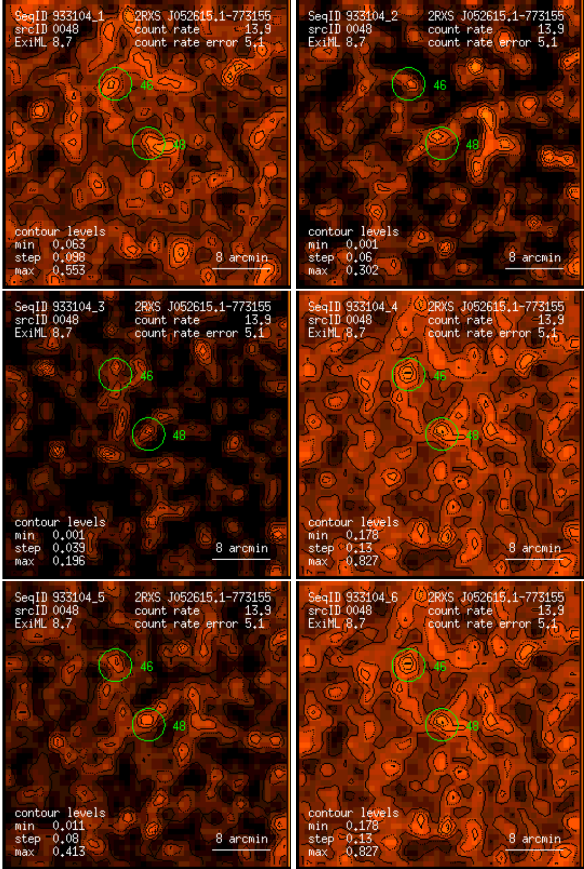
Figure 48: RASS 933104: detection 0048: band rate images, Gaussian filter: (1) PSPC channels 11 – 41, (2) 52 – 90, (3) 91 – 201, (4) 11 – 235, (5) 52 – 201, (6) 11 – 201. Broad band rates in counts/ks. Band rate contour levels in counts/ks/arcmin 2 .
