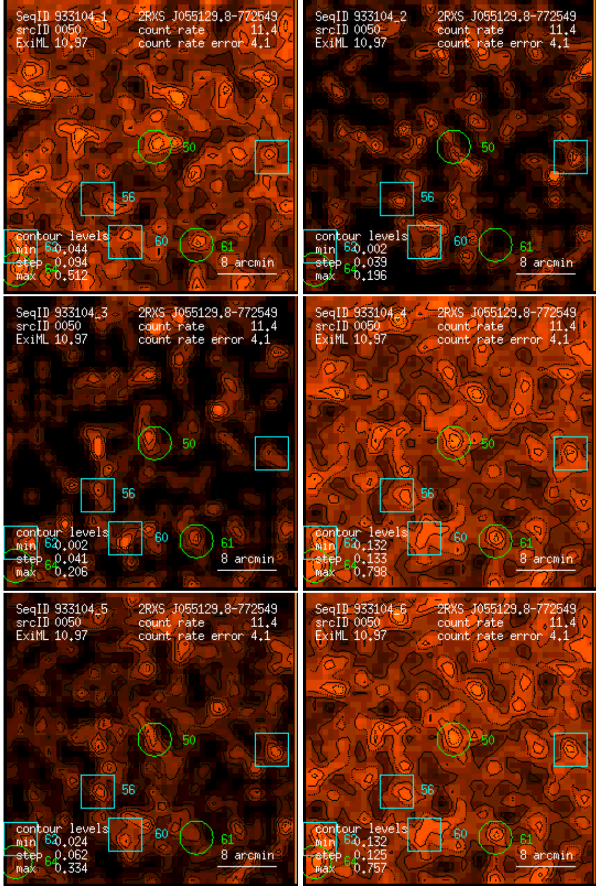
Figure 50: RASS 933104: detection 0050: band rate images, Gaussian filter: (1) PSPC channels 11 – 41, (2) 52 – 90, (3) 91 – 201, (4) 11 – 235, (5) 52 – 201, (6) 11 – 201. Broad band rates in counts/ks. Band rate contour levels in counts/ks/arcmin 2 .
