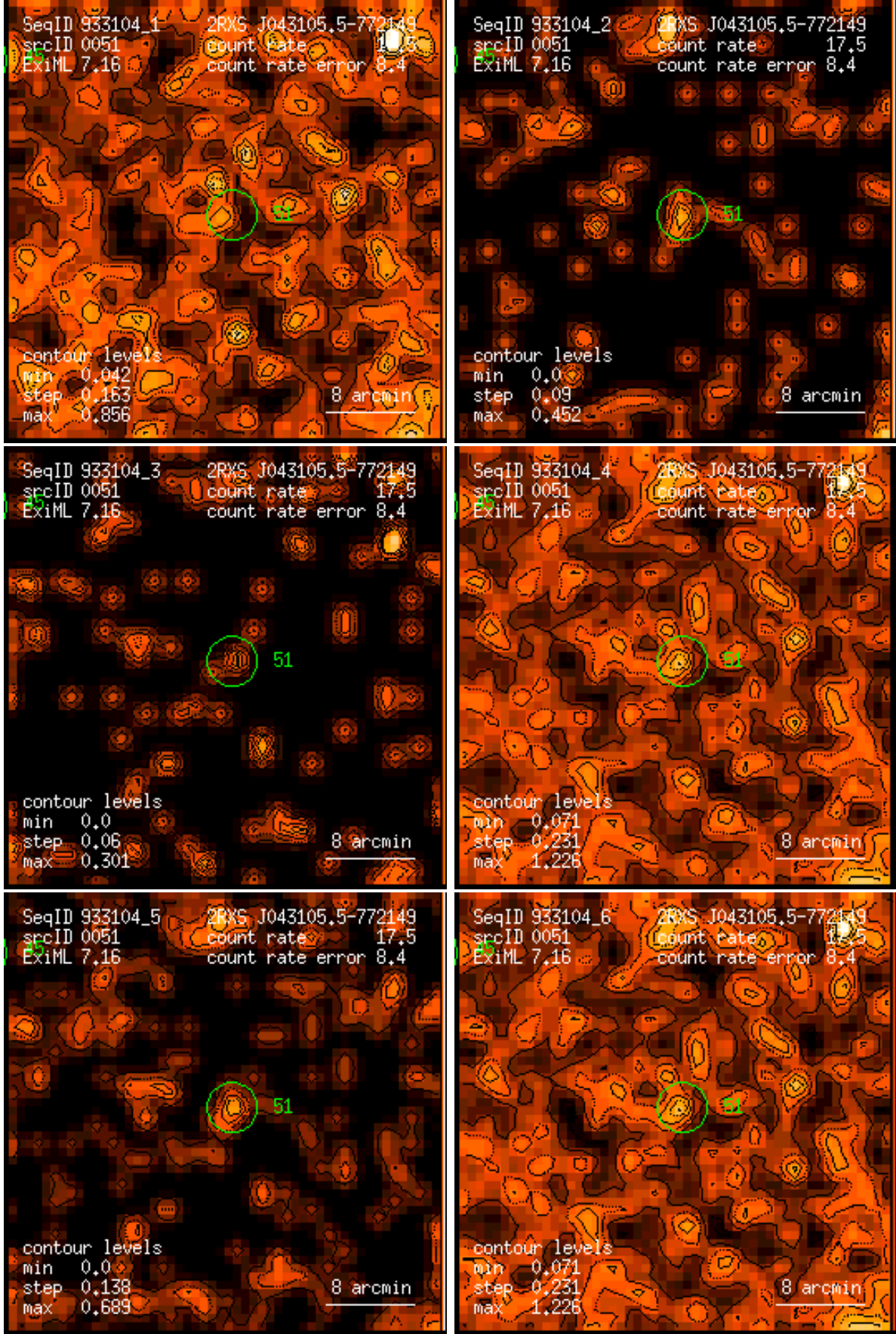
Figure 51: RASS 933104: detection 0051: band rate images, Gaussian filter: (1) PSPC channels 11 – 41, (2) 52 – 90, (3) 91 – 201, (4) 11 – 235, (5) 52 – 201, (6) 11 – 201. Broad band rates in counts/ks. Band rate contour levels in counts/ks/arcmin 2 .
