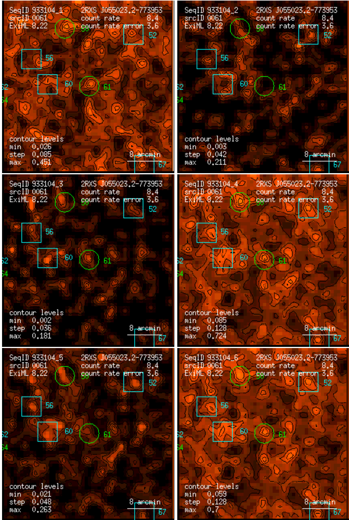
Figure 61: RASS 933104: detection 0061: band rate images, Gaussian filter: (1) PSPC channels 11 – 41, (2) 52 – 90, (3) 91 – 201, (4) 11 – 235, (5) 52 – 201, (6) 11 – 201. Broad band rates in counts/ks. Band rate contour levels in counts/ks/arcmin 2 .
