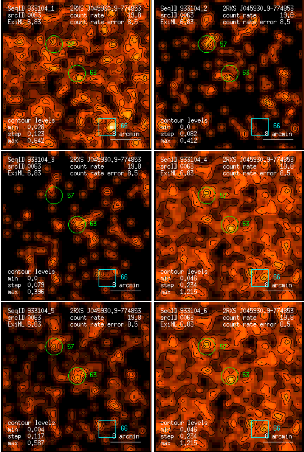
Figure 63: RASS 933104: detection 0063: band rate images, Gaussian filter: (1) PSPC channels 11 – 41, (2) 52 – 90, (3) 91 – 201, (4) 11 – 235, (5) 52 – 201, (6) 11 – 201. Broad band rates in counts/ks. Band rate contour levels in counts/ks/arcmin 2 .
