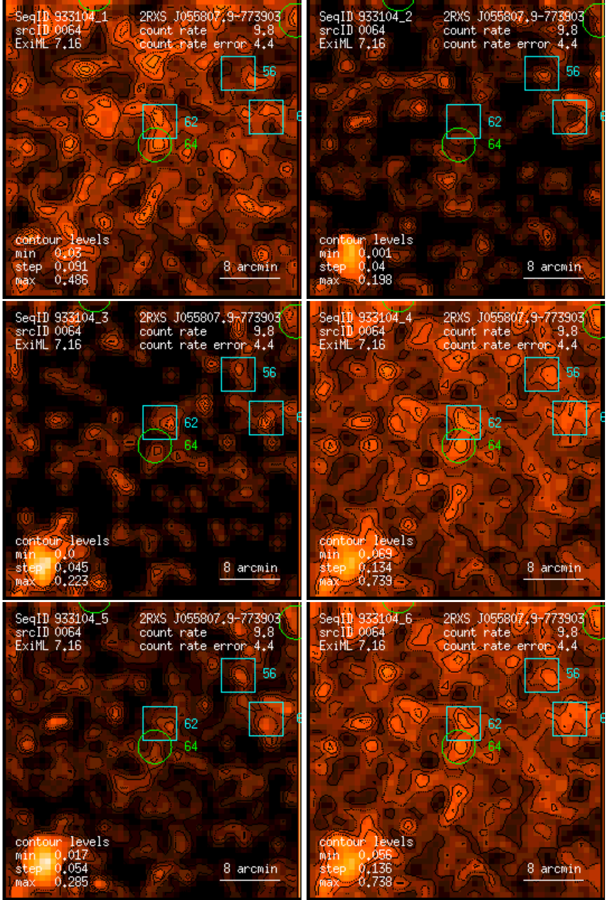
Figure 64: RASS 933104: detection 0064: band rate images, Gaussian filter: (1) PSPC channels 11 – 41, (2) 52 – 90, (3) 91 – 201, (4) 11 – 235, (5) 52 – 201, (6) 11 – 201. Broad band rates in counts/ks. Band rate contour levels in counts/ks/arcmin 2 .
