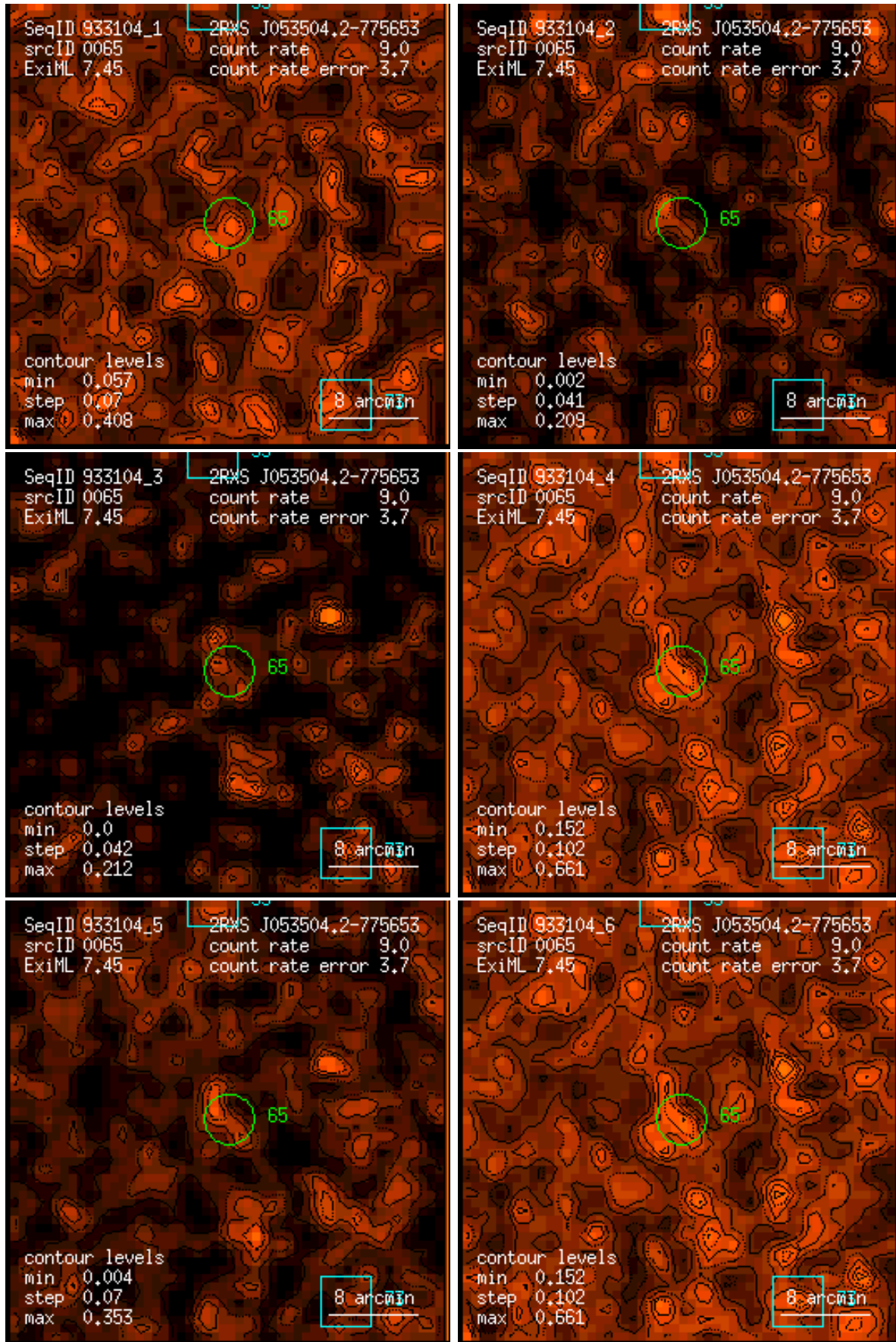
Figure 65: RASS 933104: detection 0065: band rate images, Gaussian filter: (1) PSPC channels 11 – 41, (2) 52 – 90, (3) 91 – 201, (4) 11 – 235, (5) 52 – 201, (6) 11 – 201. Broad band rates in counts/ks. Band rate contour levels in counts/ks/arcmin 2 .
