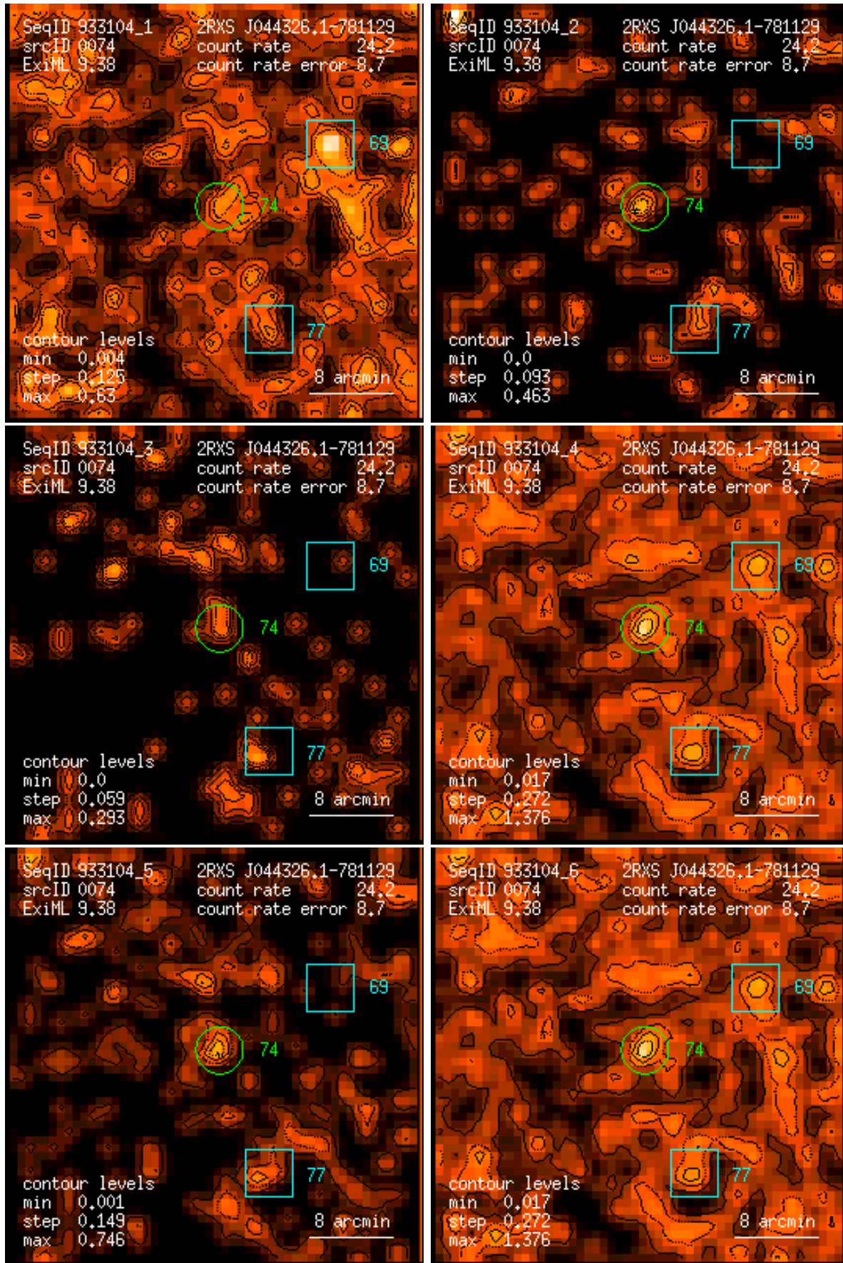
Figure 74: RASS 933104: detection 0074: band rate images, Gaussian filter: (1) PSPC channels 11 – 41, (2) 52 – 90, (3) 91 – 201, (4) 11 – 235, (5) 52 – 201, (6) 11 – 201. Broad band rates in counts/ks. Band rate contour levels in counts/ks/arcmin 2 .
