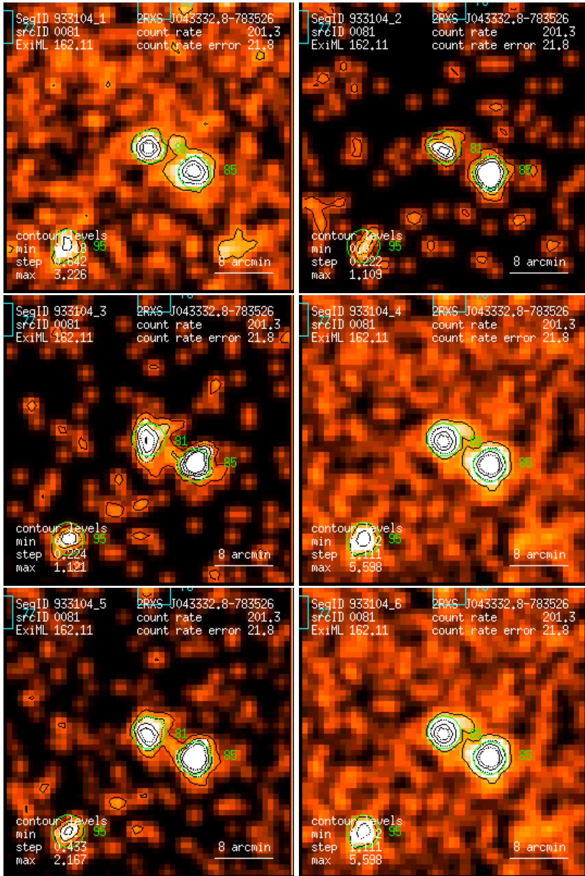
Figure 81: RASS 933104: detection 0081: band rate images, Gaussian filter: (1) PSPC channels 11 – 41, (2) 52 – 90, (3) 91 – 201, (4) 11 – 235, (5) 52 – 201, (6) 11 – 201. Broad band rates in counts/ks. Band rate contour levels in counts/ks/arcmin 2 .
