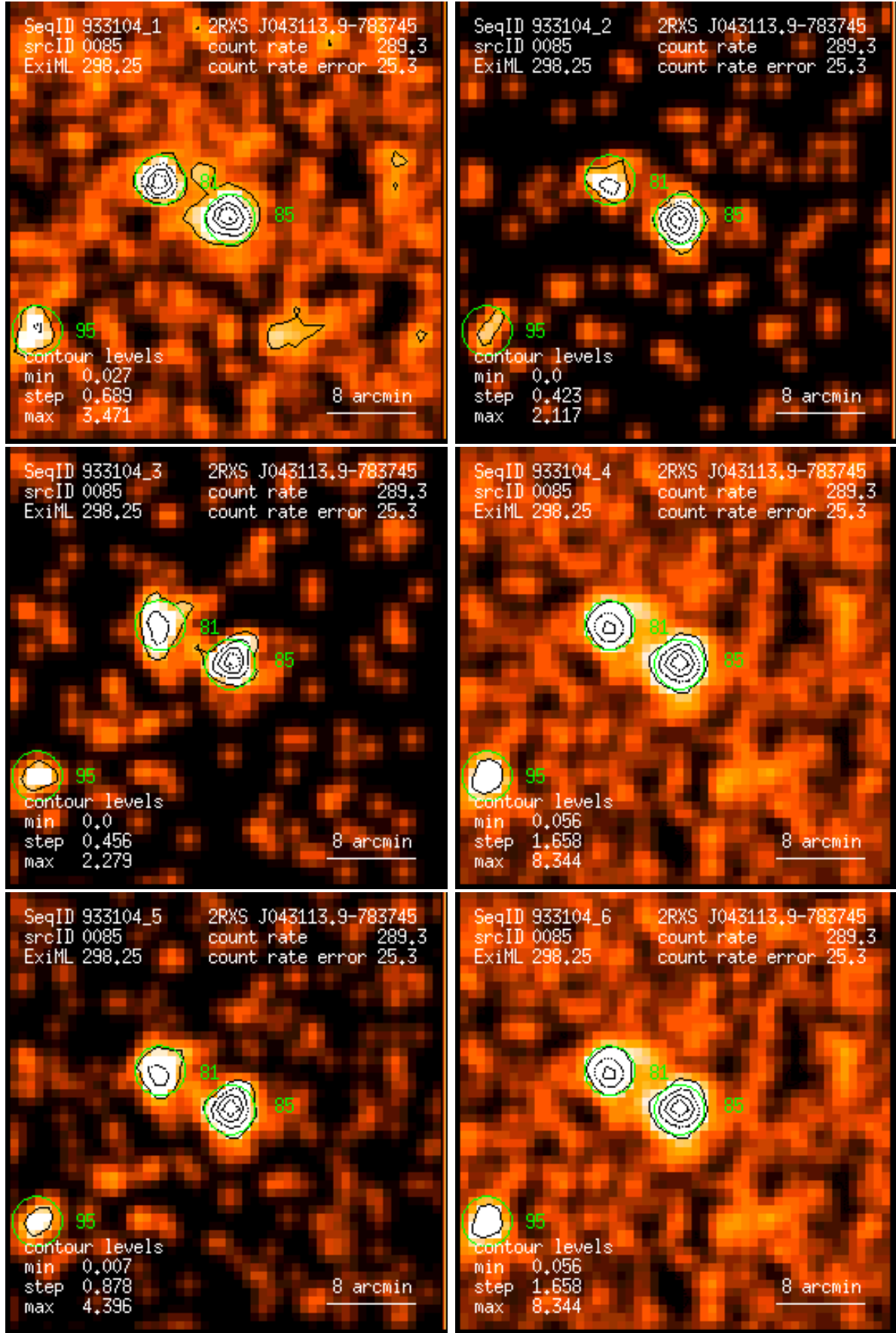
Figure 85: RASS 933104: detection 0085: band rate images, Gaussian filter: (1) PSPC channels 11 – 41, (2) 52 – 90, (3) 91 – 201, (4) 11 – 235, (5) 52 – 201, (6) 11 – 201. Broad band rates in counts/ks. Band rate contour levels in counts/ks/arcmin 2 .
