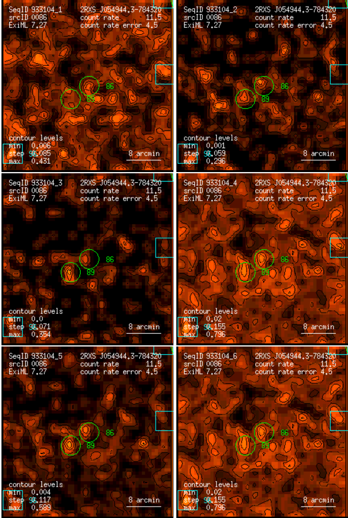
Figure 86: RASS 933104: detection 0086: band rate images, Gaussian filter: (1) PSPC channels 11 – 41, (2) 52 – 90, (3) 91 – 201, (4) 11 – 235, (5) 52 – 201, (6) 11 – 201. Broad band rates in counts/ks. Band rate contour levels in counts/ks/arcmin 2 .
