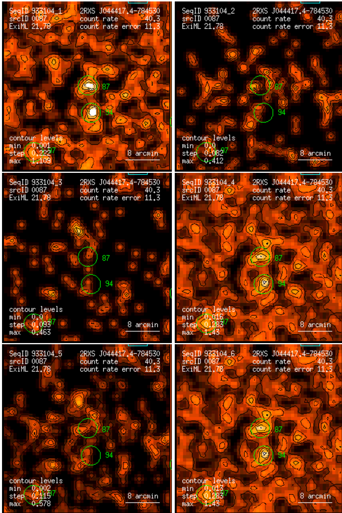
Figure 87: RASS 933104: detection 0087: band rate images, Gaussian filter: (1) PSPC channels 11 – 41, (2) 52 – 90, (3) 91 – 201, (4) 11 – 235, (5) 52 – 201, (6) 11 – 201. Broad band rates in counts/ks. Band rate contour levels in counts/ks/arcmin 2 .
