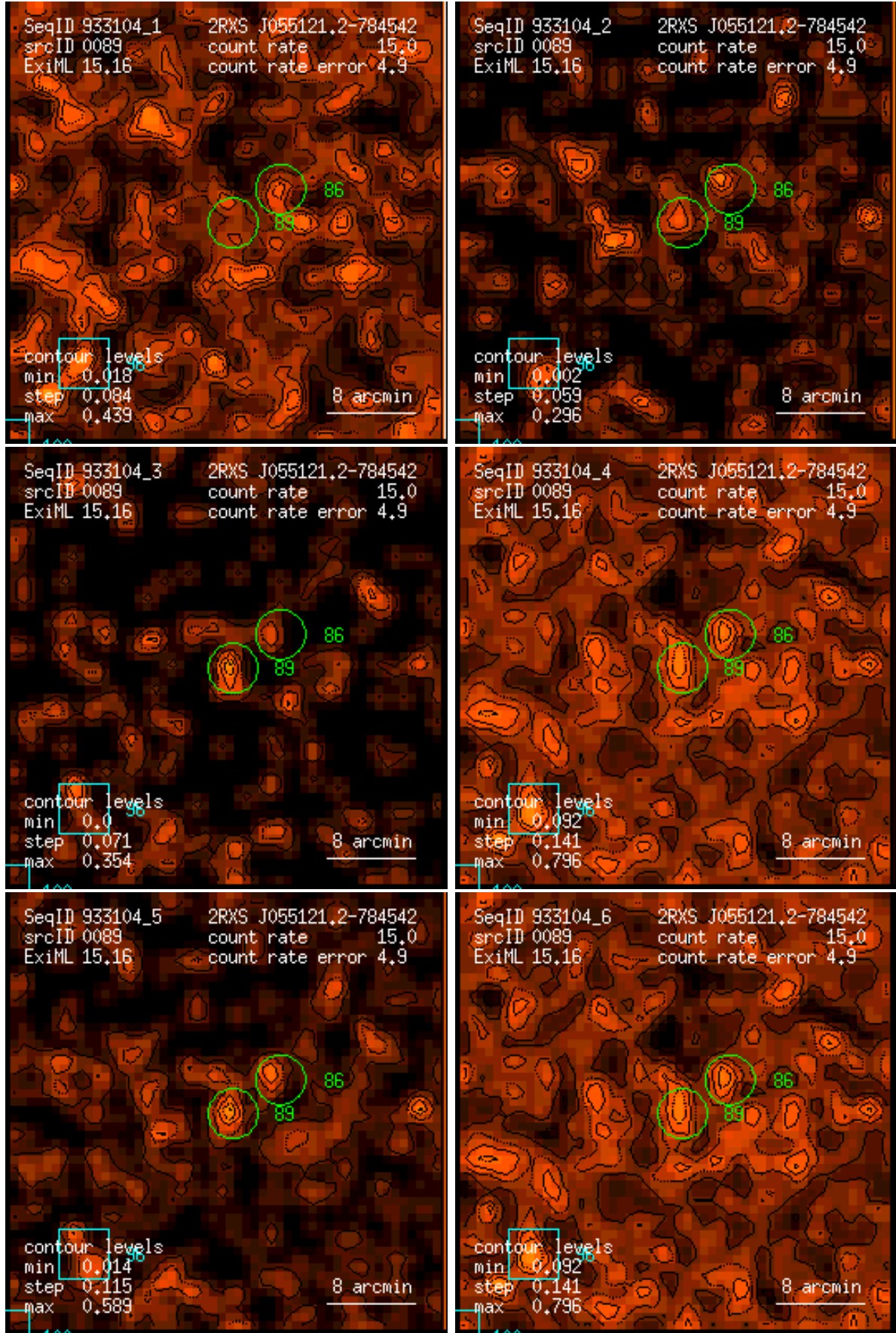
Figure 89: RASS 933104: detection 0089: band rate images, Gaussian filter: (1) PSPC channels 11 – 41, (2) 52 – 90, (3) 91 – 201, (4) 11 – 235, (5) 52 – 201, (6) 11 – 201. Broad band rates in counts/ks. Band rate contour levels in counts/ks/arcmin 2 .
