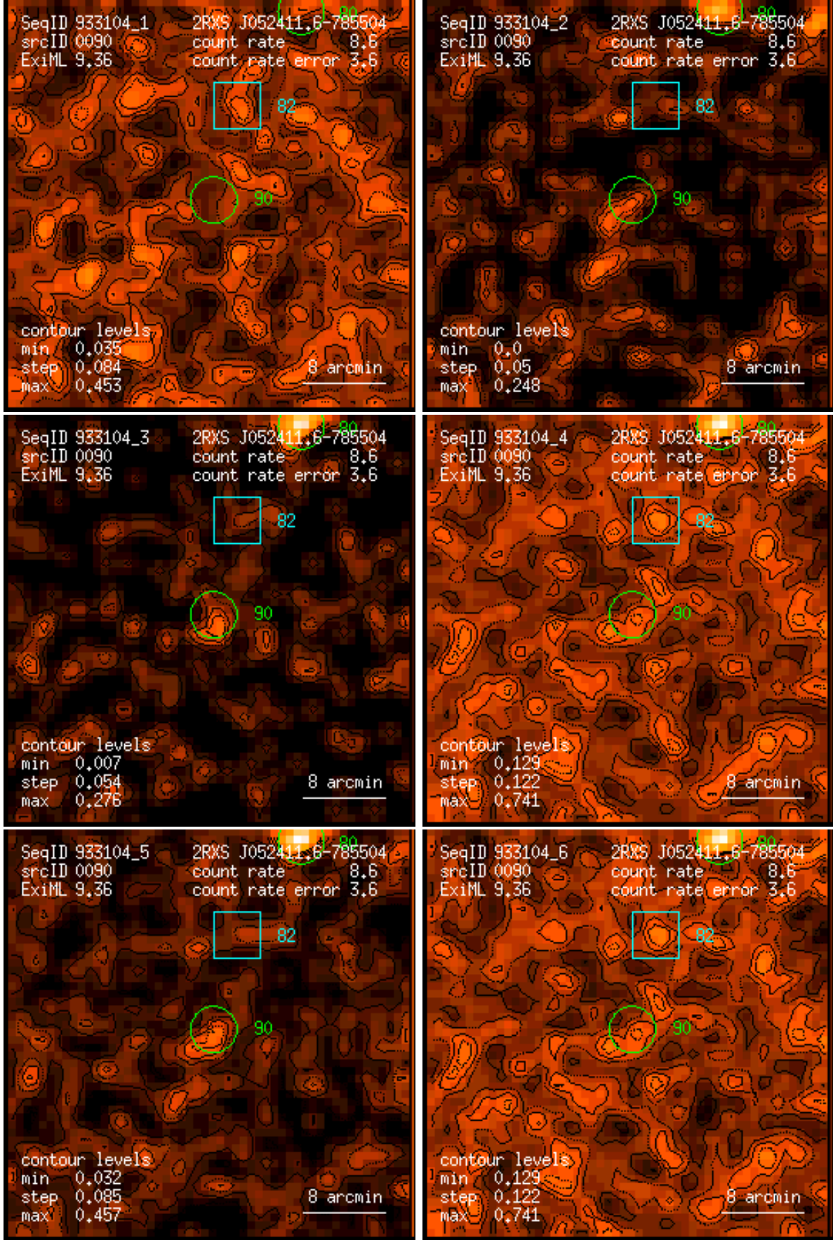
Figure 90: RASS 933104: detection 0090: band rate images, Gaussian filter: (1) PSPC channels 11 – 41, (2) 52 – 90, (3) 91 – 201, (4) 11 – 235, (5) 52 – 201, (6) 11 – 201. Broad band rates in counts/ks. Band rate contour levels in counts/ks/arcmin 2 .
