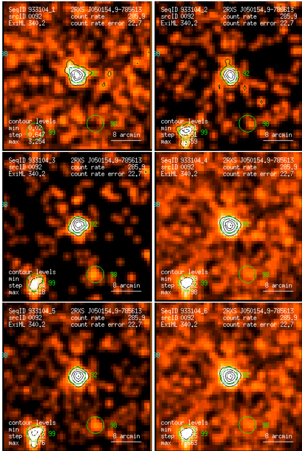
Figure 92: RASS 933104: detection 0092: band rate images, Gaussian filter: (1) PSPC channels 11 – 41, (2) 52 – 90, (3) 91 – 201, (4) 11 – 235, (5) 52 – 201, (6) 11 – 201. Broad band rates in counts/ks. Band rate contour levels in counts/ks/arcmin 2 .
