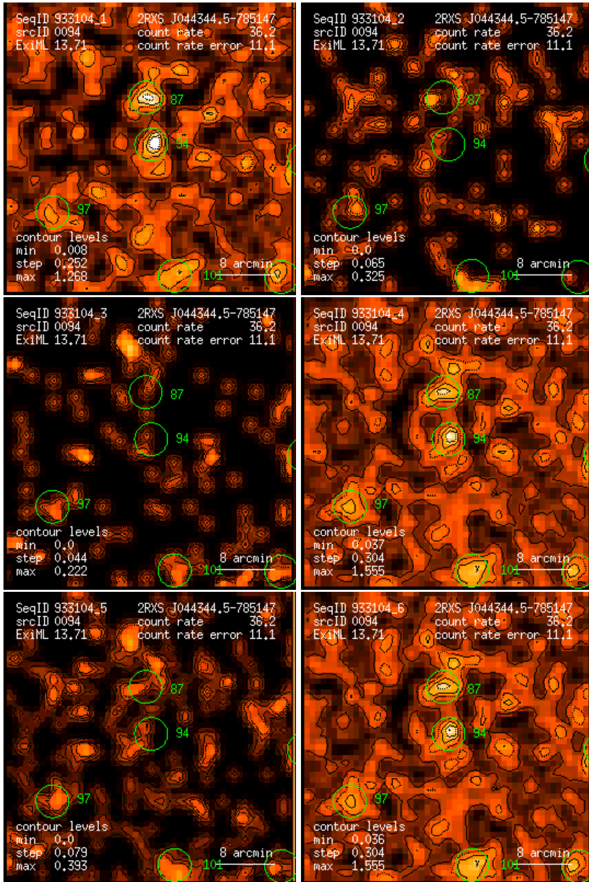
Figure 94: RASS 933104: detection 0094: band rate images, Gaussian filter: (1) PSPC channels 11 – 41, (2) 52 – 90, (3) 91 – 201, (4) 11 – 235, (5) 52 – 201, (6) 11 – 201. Broad band rates in counts/ks. Band rate contour levels in counts/ks/arcmin 2 .
